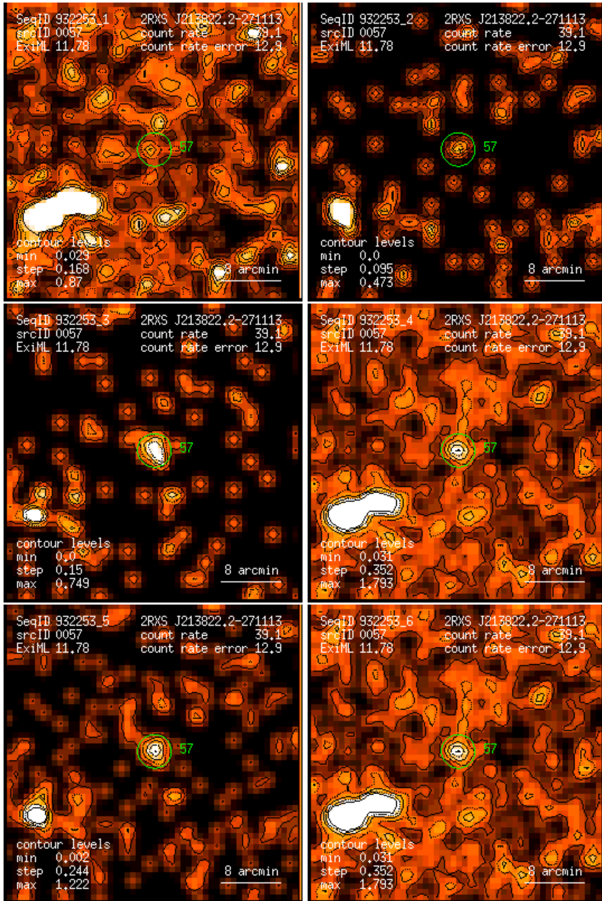
Figure 57: RASS 932253: detection 0057: band rate images, Gaussian filter: (1) PSPC channels 11 – 41, (2) 52 – 90, (3) 91 – 201, (4) 11 – 235, (5) 52 – 201, (6) 11 – 201. Broad band rates in counts/ks. Band rate contour levels in counts/ks/arcmin 2 .
