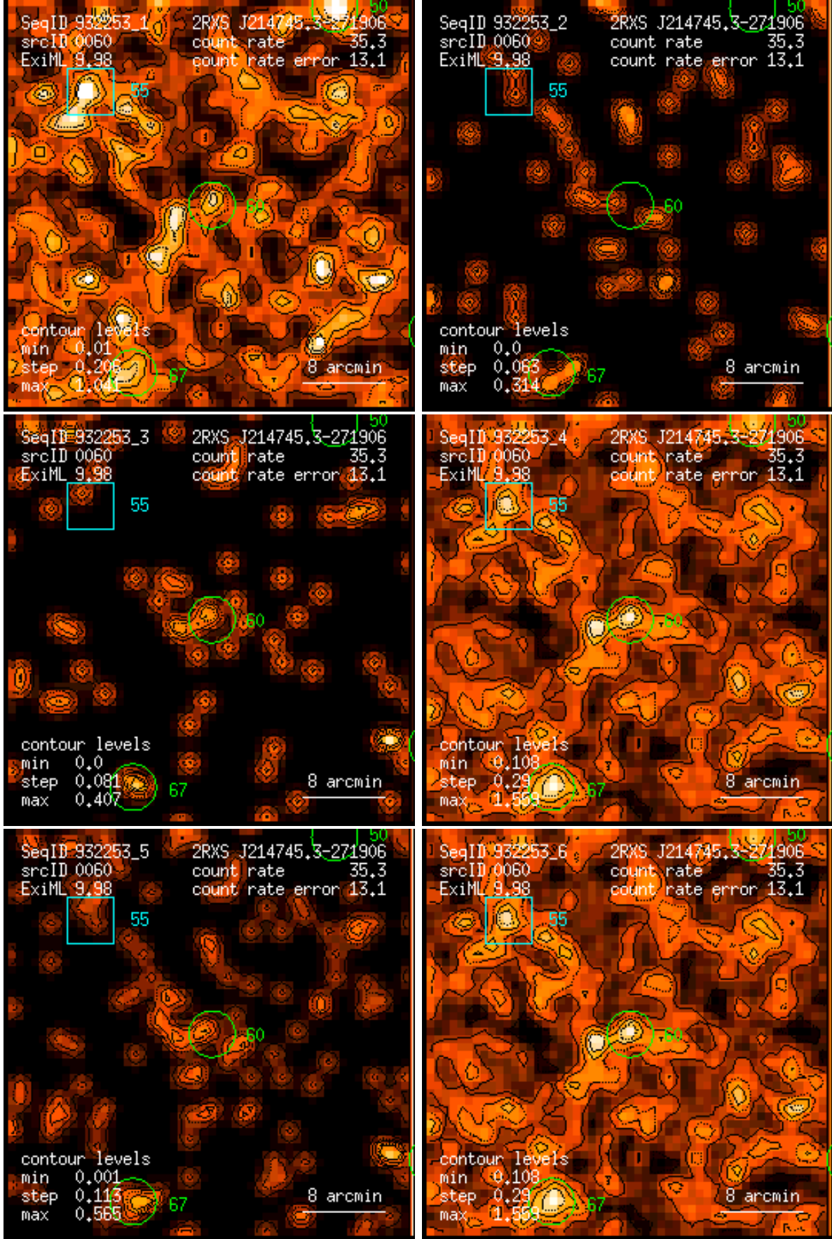
Figure 60: RASS 932253: detection 0060: band rate images, Gaussian filter: (1) PSPC channels 11 – 41, (2) 52 – 90, (3) 91 – 201, (4) 11 – 235, (5) 52 – 201, (6) 11 – 201. Broad band rates in counts/ks. Band rate contour levels in counts/ks/arcmin 2 .
