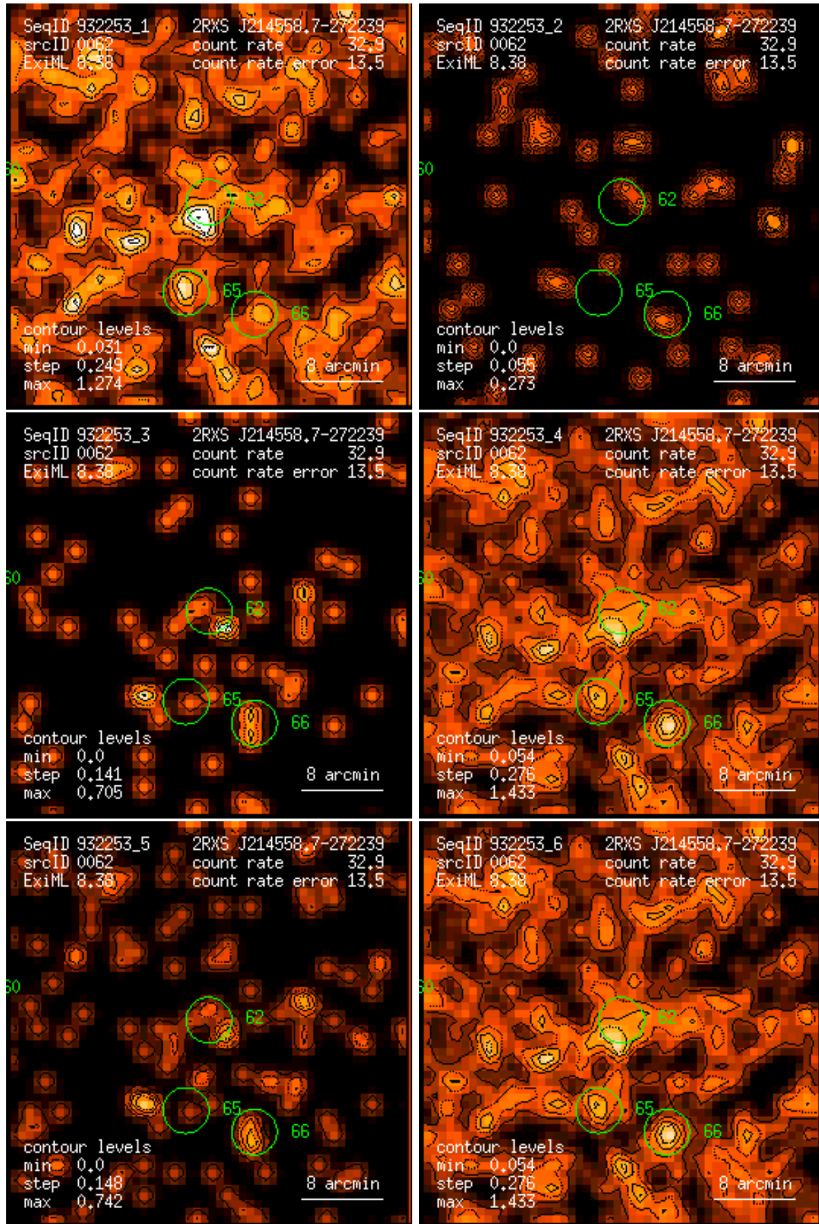
Figure 62: RASS 932253: detection 0062: band rate images, Gaussian filter: (1) PSPC channels 11 – 41, (2) 52 – 90, (3) 91 – 201, (4) 11 – 235, (5) 52 – 201, (6) 11 – 201. Broad band rates in counts/ks. Band rate contour levels in counts/ks/arcmin 2 .
