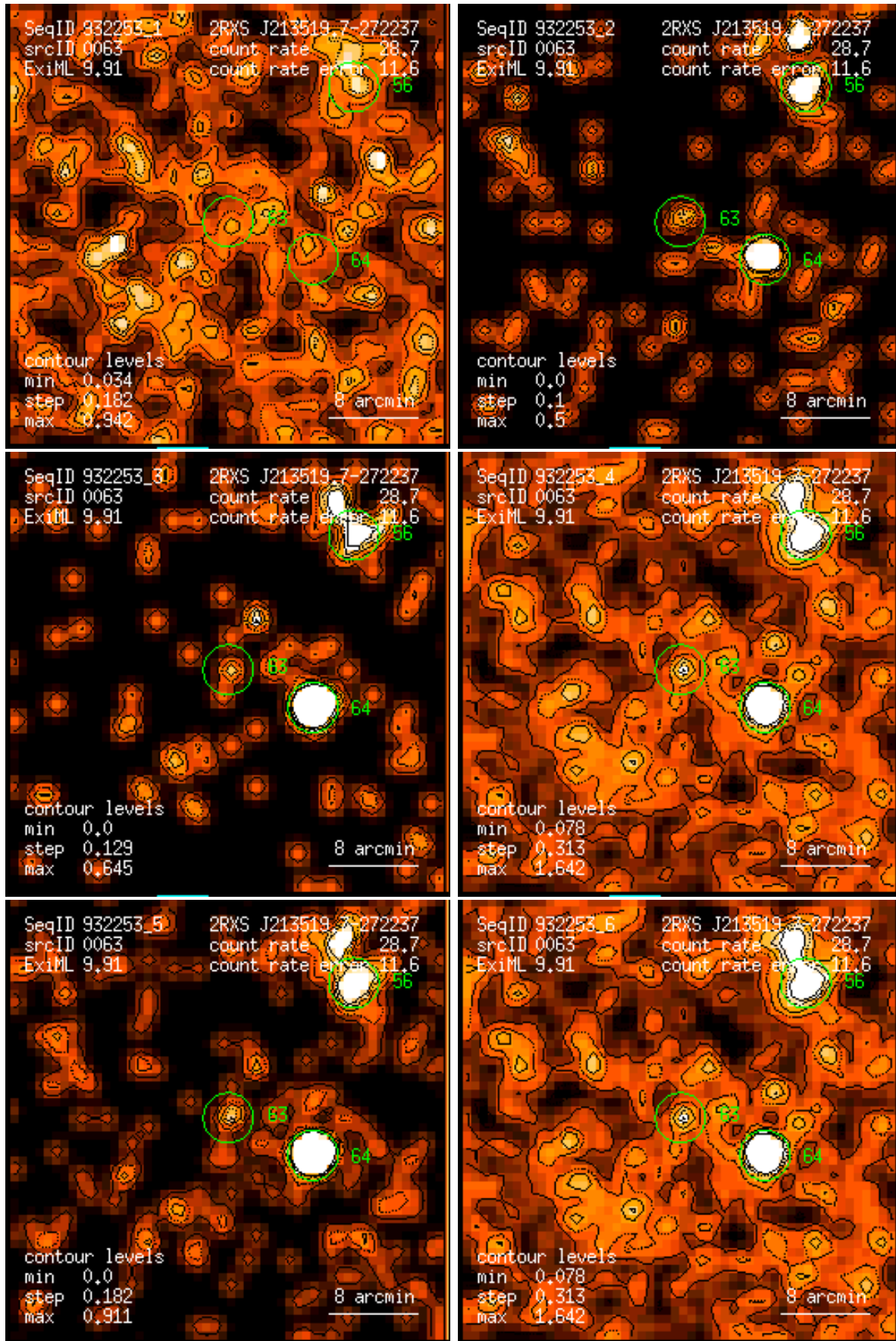
Figure 63: RASS 932253: detection 0063: band rate images, Gaussian filter: (1) PSPC channels 11 – 41, (2) 52 – 90, (3) 91 – 201, (4) 11 – 235, (5) 52 – 201, (6) 11 – 201. Broad band rates in counts/ks. Band rate contour levels in counts/ks/arcmin 2 .
