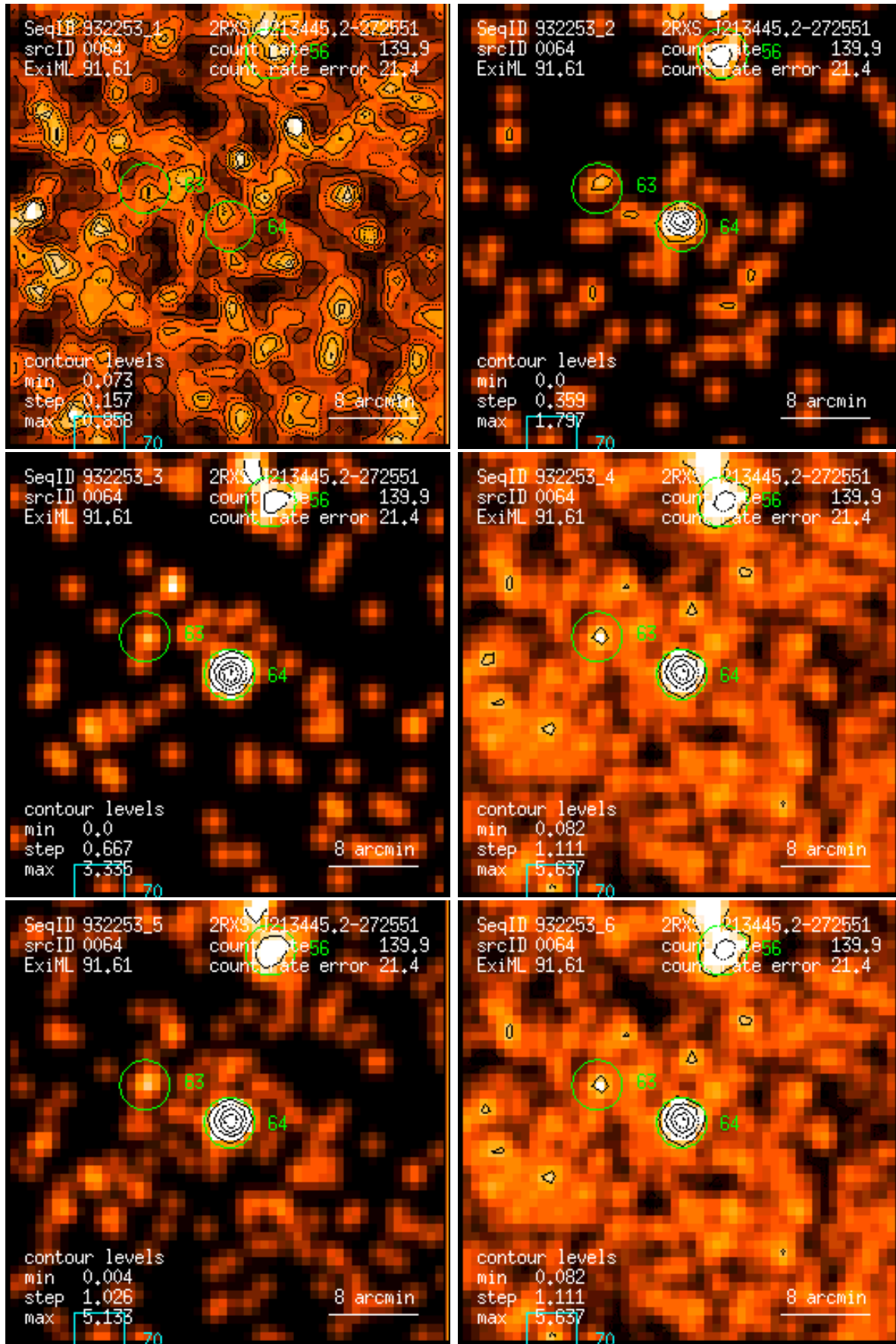
Figure 64: RASS 932253: detection 0064: band rate images, Gaussian filter: (1) PSPC channels 11 – 41, (2) 52 – 90, (3) 91 – 201, (4) 11 – 235, (5) 52 – 201, (6) 11 – 201. Broad band rates in counts/ks. Band rate contour levels in counts/ks/arcmin 2 .
