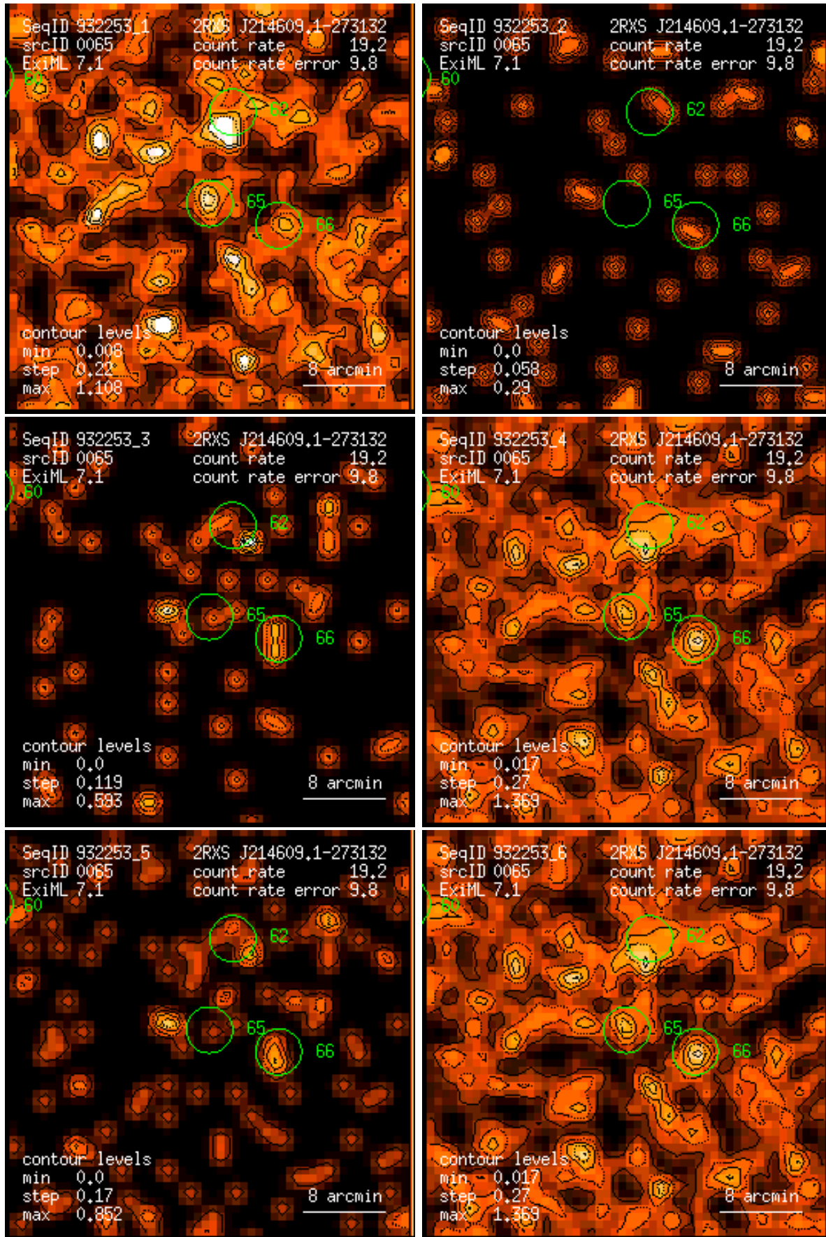
Figure 65: RASS 932253: detection 0065: band rate images, Gaussian filter: (1) PSPC channels 11 – 41, (2) 52 – 90, (3) 91 – 201, (4) 11 – 235, (5) 52 – 201, (6) 11 – 201. Broad band rates in counts/ks. Band rate contour levels in counts/ks/arcmin 2 .
