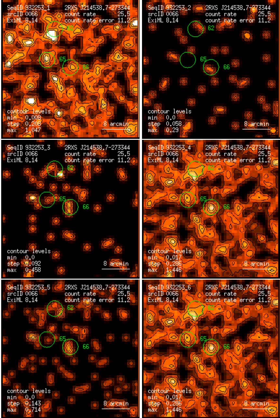
Figure 66: RASS 932253: detection 0066: band rate images, Gaussian filter: (1) PSPC channels 11 – 41, (2) 52 – 90, (3) 91 – 201, (4) 11 – 235, (5) 52 – 201, (6) 11 – 201. Broad band rates in counts/ks. Band rate contour levels in counts/ks/arcmin 2 .
