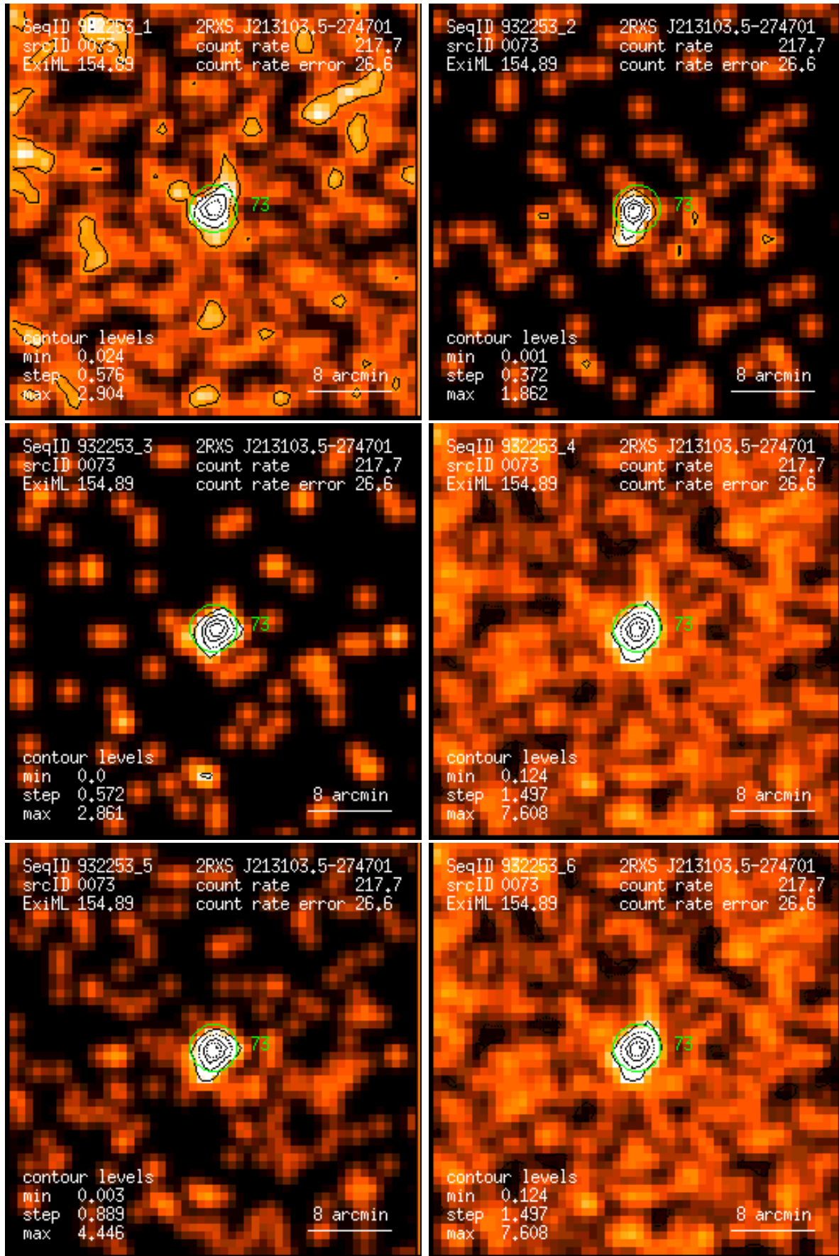
Figure 73: RASS 932253: detection 0073: band rate images, Gaussian filter: (1) PSPC channels 11 – 41, (2) 52 – 90, (3) 91 – 201, (4) 11 – 235, (5) 52 – 201, (6) 11 – 201. Broad band rates in counts/ks. Band rate contour levels in counts/ks/arcmin 2 .
