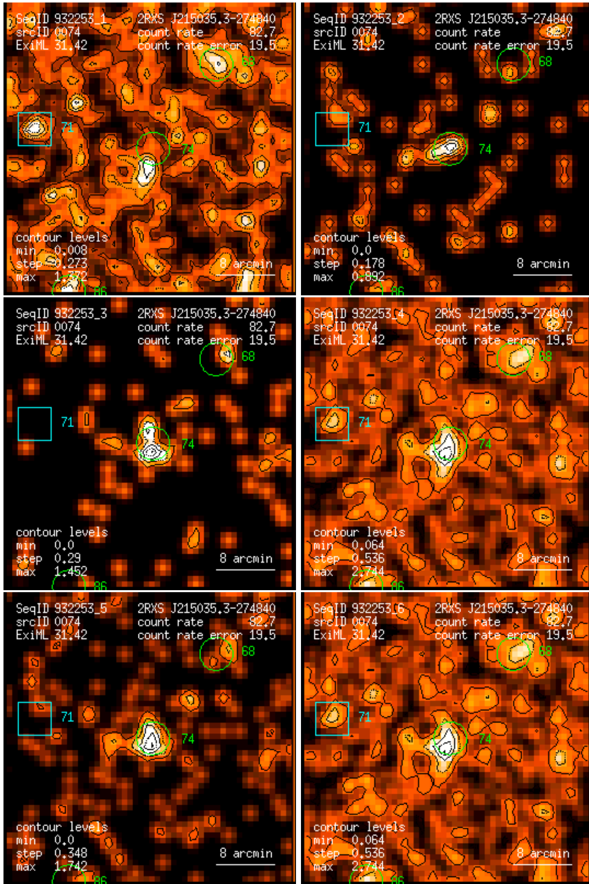
Figure 74: RASS 932253: detection 0074: band rate images, Gaussian filter: (1) PSPC channels 11 – 41, (2) 52 – 90, (3) 91 – 201, (4) 11 – 235, (5) 52 – 201, (6) 11 – 201. Broad band rates in counts/ks. Band rate contour levels in counts/ks/arcmin 2 .
