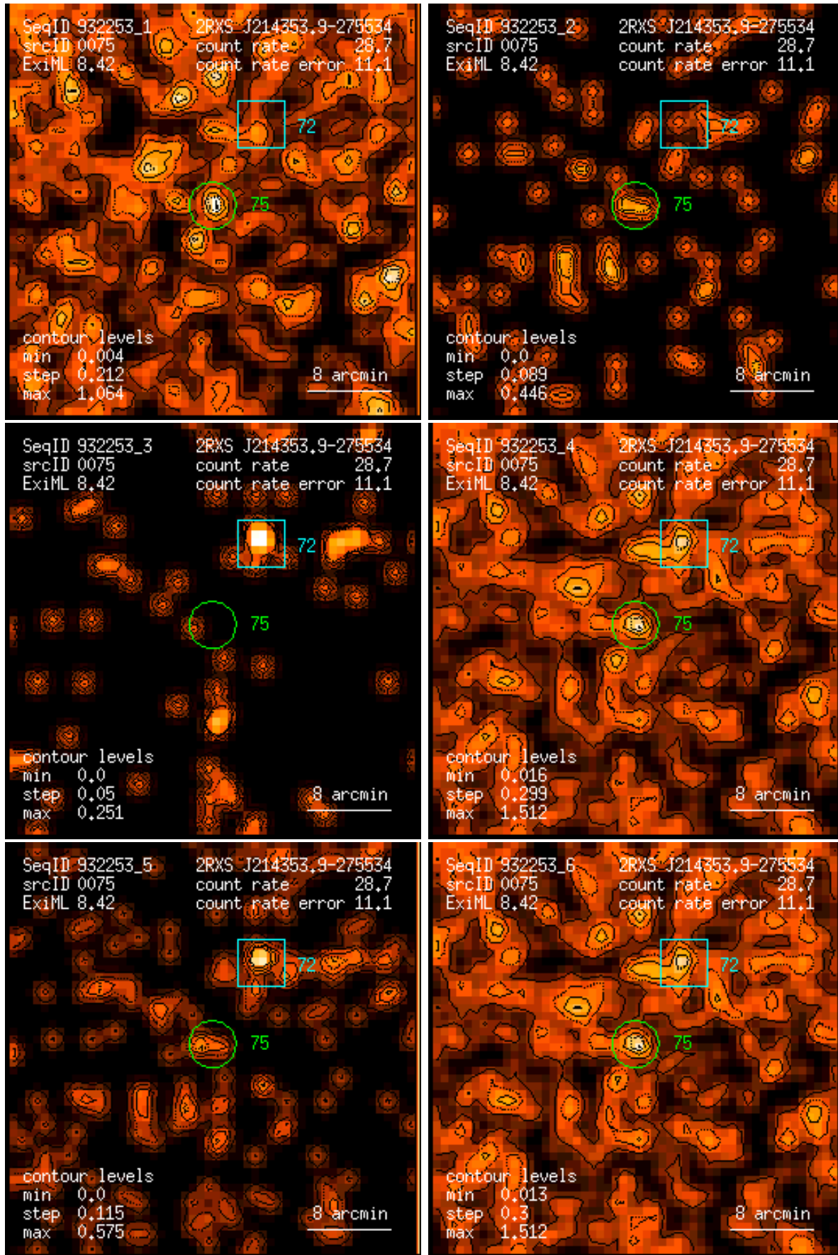
Figure 75: RASS 932253: detection 0075: band rate images, Gaussian filter: (1) PSPC channels 11 – 41, (2) 52 – 90, (3) 91 – 201, (4) 11 – 235, (5) 52 – 201, (6) 11 – 201. Broad band rates in counts/ks. Band rate contour levels in counts/ks/arcmin 2 .
