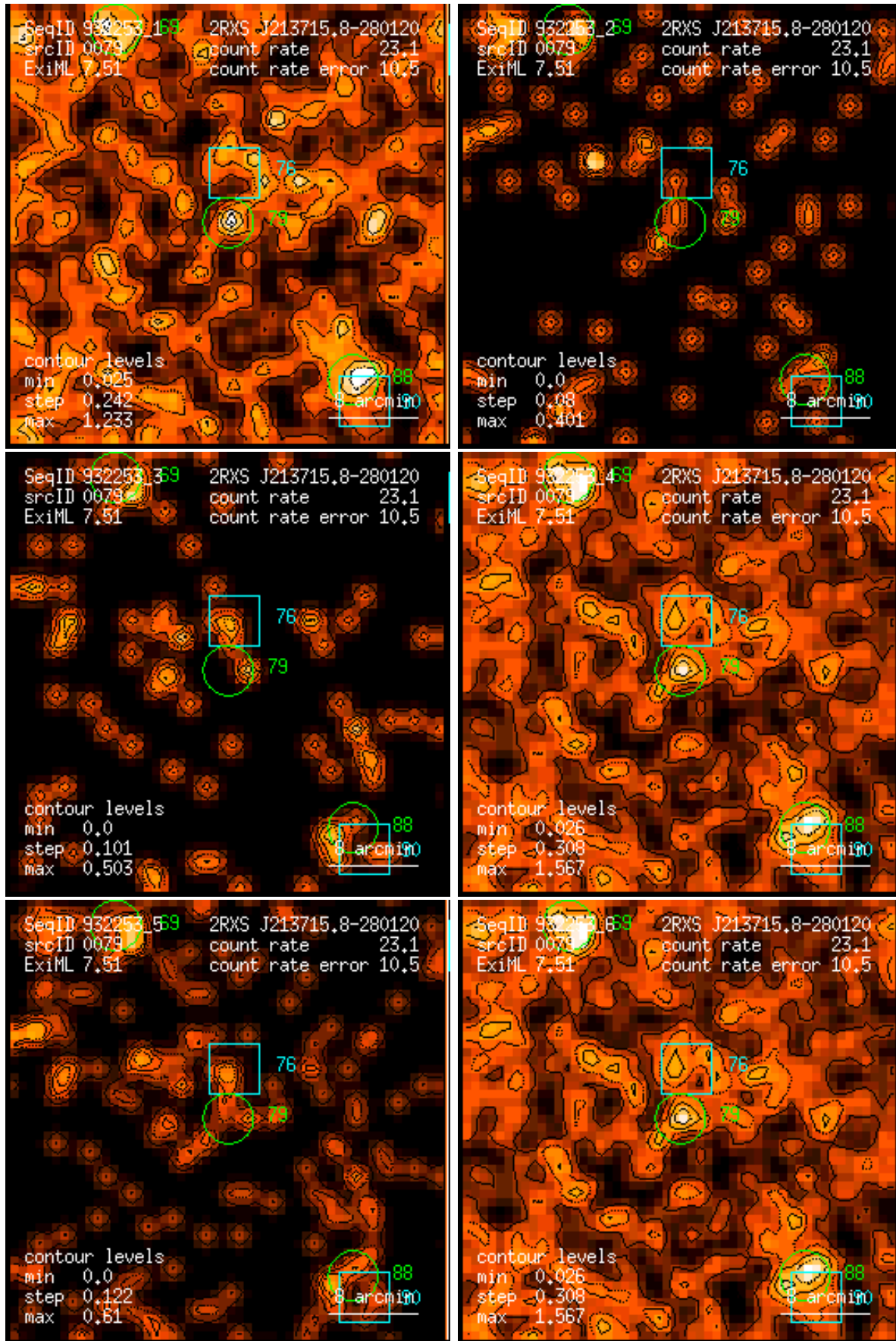
Figure 79: RASS 932253: detection 0079: band rate images, Gaussian filter: (1) PSPC channels 11 – 41, (2) 52 – 90, (3) 91 – 201, (4) 11 – 235, (5) 52 – 201, (6) 11 – 201. Broad band rates in counts/ks. Band rate contour levels in counts/ks/arcmin 2 .
