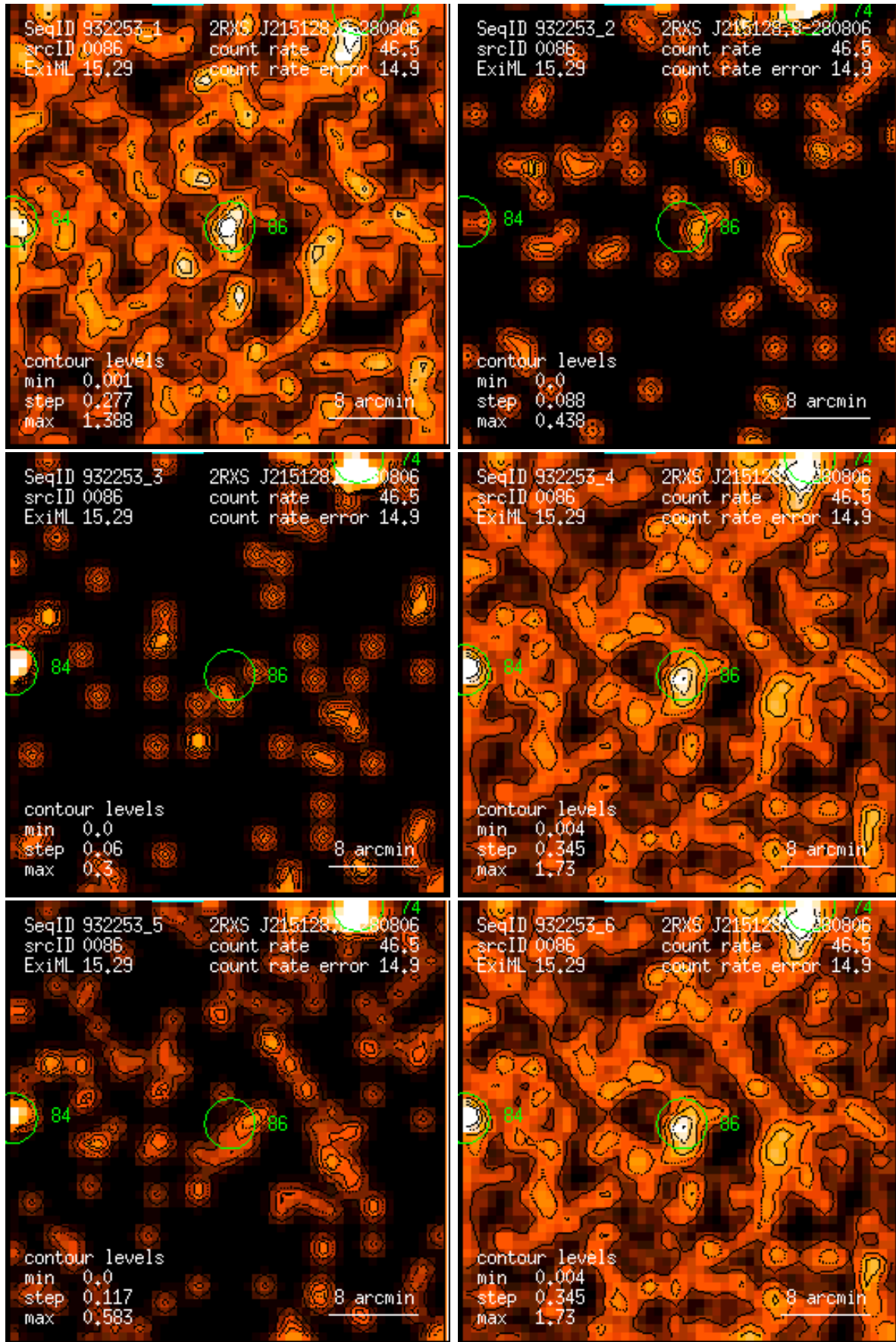
Figure 86: RASS 932253: detection 0086: band rate images, Gaussian filter: (1) PSPC channels 11 – 41, (2) 52 – 90, (3) 91 – 201, (4) 11 – 235, (5) 52 – 201, (6) 11 – 201. Broad band rates in counts/ks. Band rate contour levels in counts/ks/arcmin 2 .
