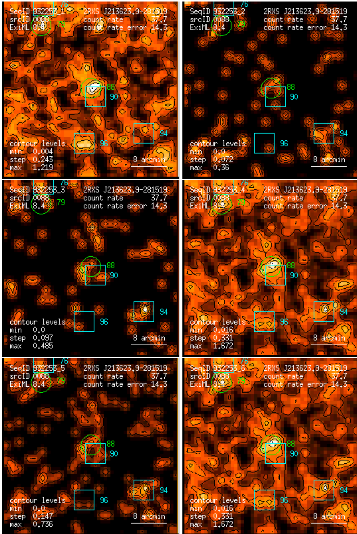
Figure 88: RASS 932253: detection 0088: band rate images, Gaussian filter: (1) PSPC channels 11 – 41, (2) 52 – 90, (3) 91 – 201, (4) 11 – 235, (5) 52 – 201, (6) 11 – 201. Broad band rates in counts/ks. Band rate contour levels in counts/ks/arcmin 2 .
