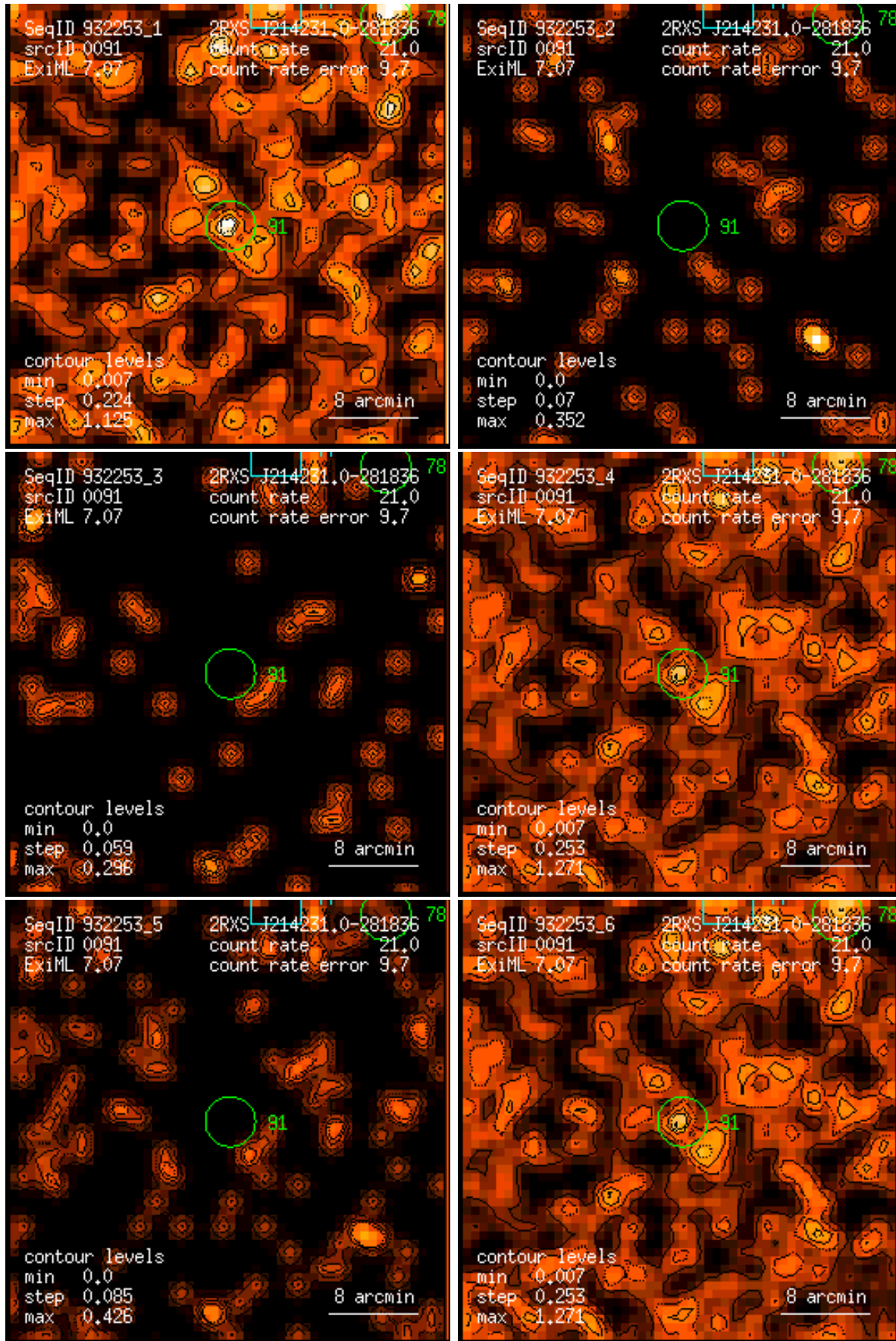
Figure 91: RASS 932253: detection 0091: band rate images, Gaussian filter: (1) PSPC channels 11 – 41, (2) 52 – 90, (3) 91 – 201, (4) 11 – 235, (5) 52 – 201, (6) 11 – 201. Broad band rates in counts/ks. Band rate contour levels in counts/ks/arcmin 2 .
