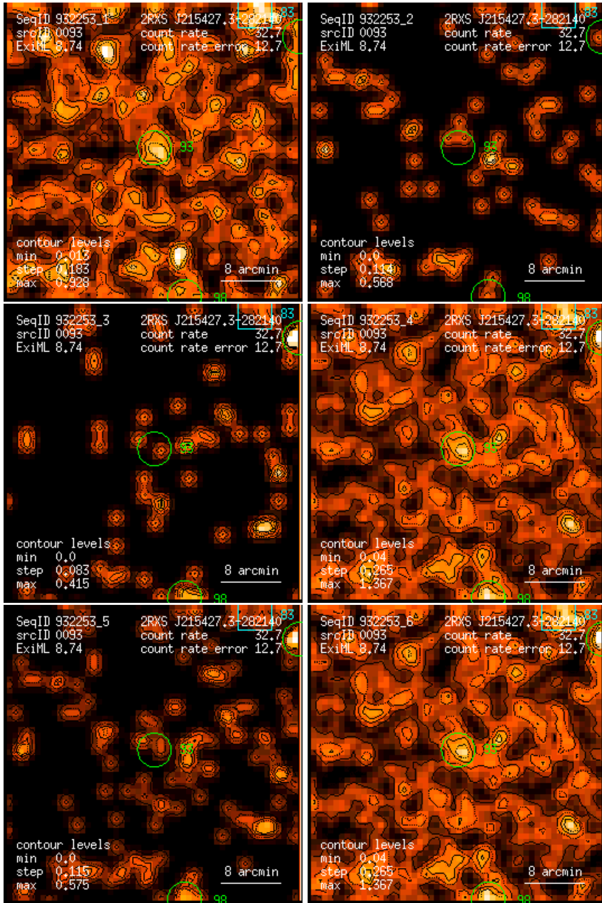
Figure 93: RASS 932253: detection 0093: band rate images, Gaussian filter: (1) PSPC channels 11 – 41, (2) 52 – 90, (3) 91 – 201, (4) 11 – 235, (5) 52 – 201, (6) 11 – 201. Broad band rates in counts/ks. Band rate contour levels in counts/ks/arcmin 2 .
