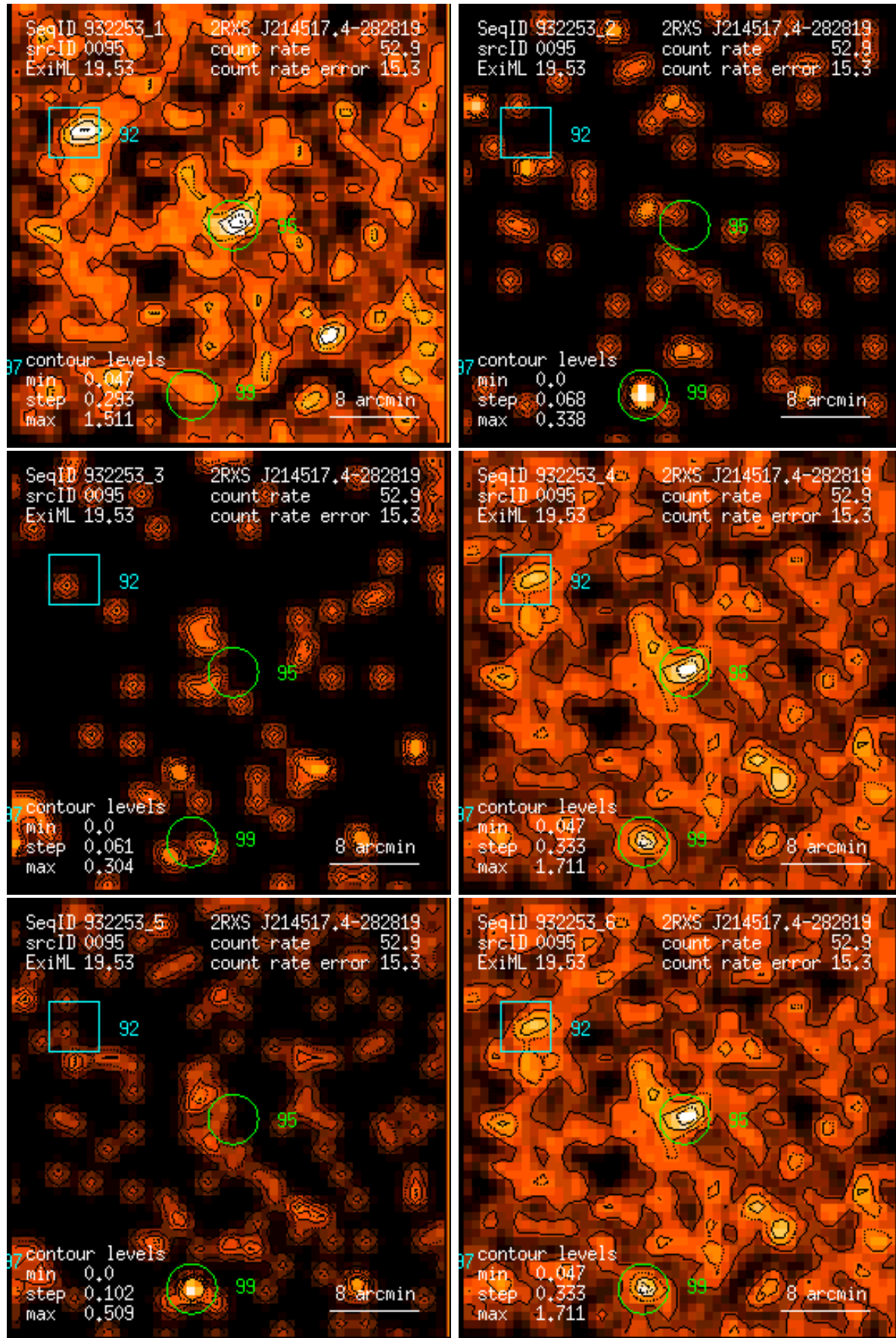
Figure 95: RASS 932253: detection 0095: band rate images, Gaussian filter: (1) PSPC channels 11 – 41, (2) 52 – 90, (3) 91 – 201, (4) 11 – 235, (5) 52 – 201, (6) 11 – 201. Broad band rates in counts/ks. Band rate contour levels in counts/ks/arcmin 2 .
