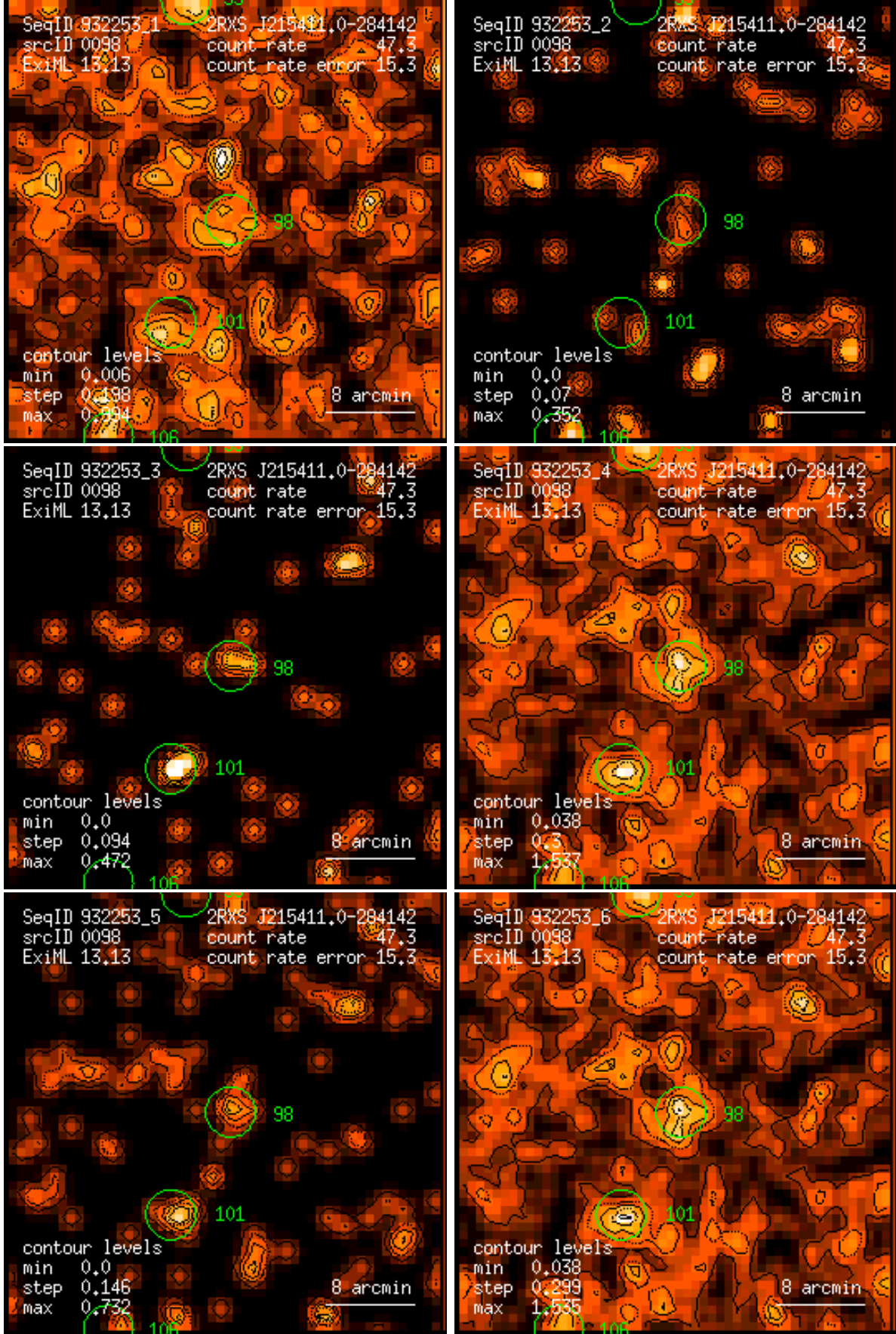
Figure 98: RASS 932253: detection 0098: band rate images, Gaussian filter: (1) PSPC channels 11 – 41, (2) 52 – 90, (3) 91 – 201, (4) 11 – 235, (5) 52 – 201, (6) 11 – 201. Broad band rates in counts/ks. Band rate contour levels in counts/ks/arcmin 2 .
