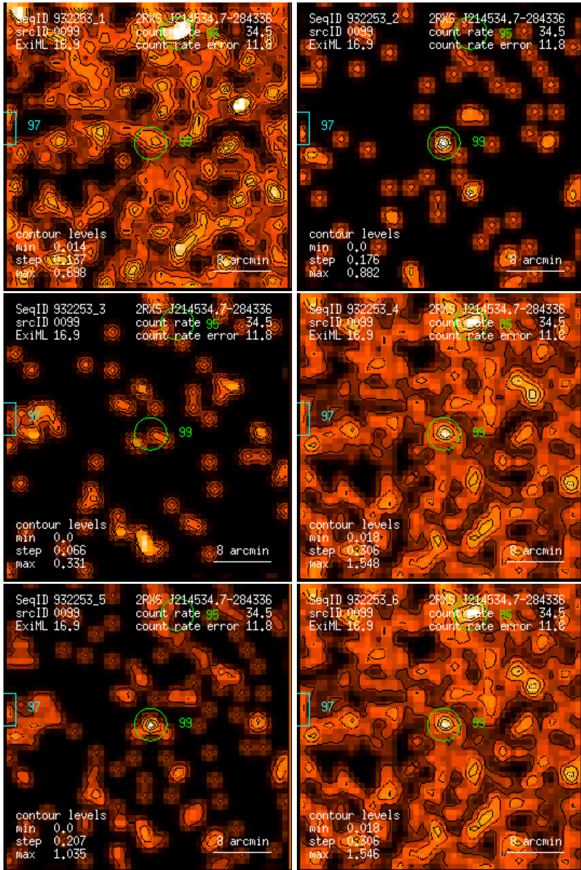
Figure 99: RASS 932253: detection 0099: band rate images, Gaussian filter: (1) PSPC channels 11 – 41, (2) 52 – 90, (3) 91 – 201, (4) 11 – 235, (5) 52 – 201, (6) 11 – 201. Broad band rates in counts/ks. Band rate contour levels in counts/ks/arcmin 2 .
