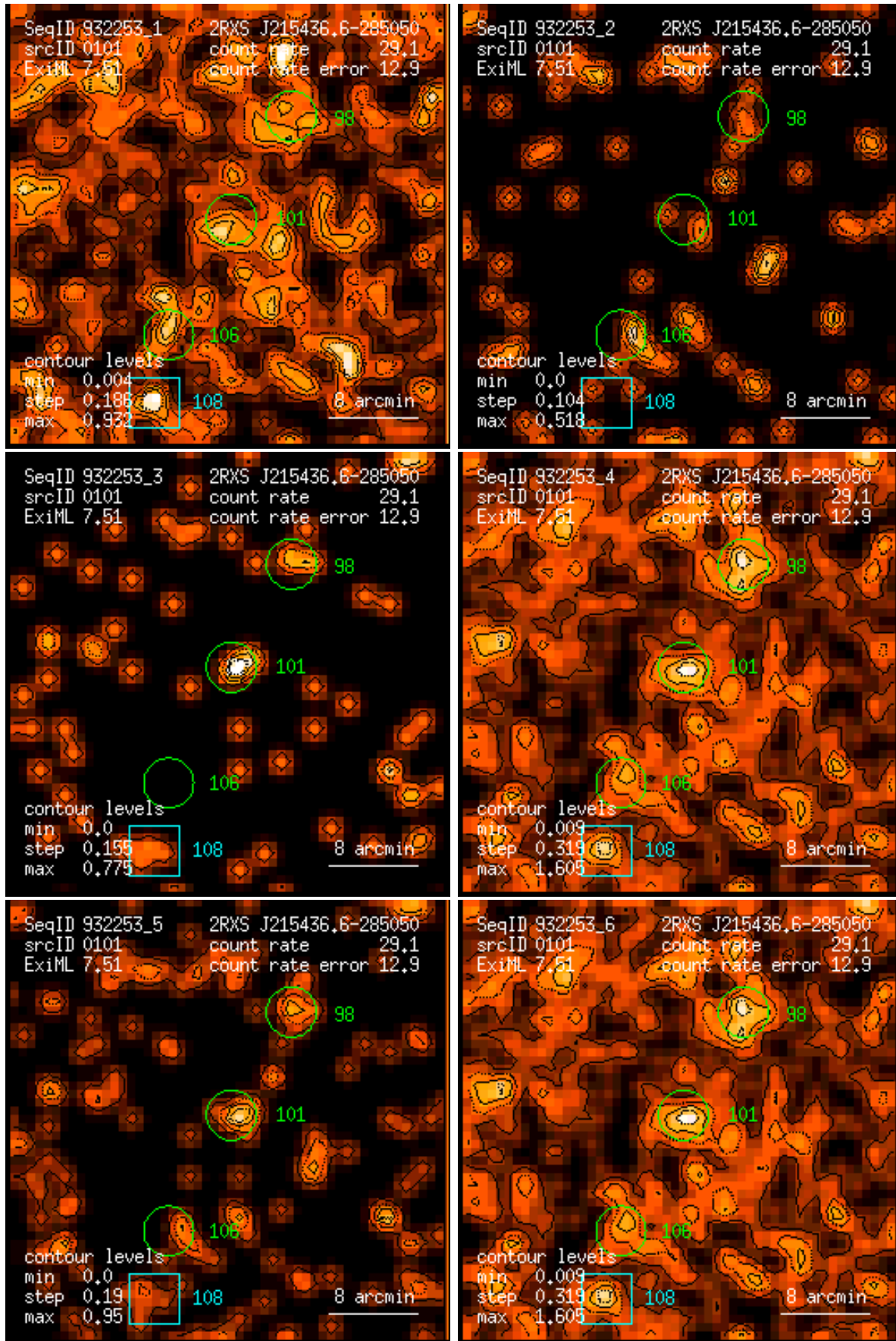
Figure 101: RASS 932253: detection 0101: band rate images, Gaussian filter: (1) PSPC channels 11 – 41, (2) 52 – 90, (3) 91 – 201, (4) 11 – 235, (5) 52 – 201, (6) 11 – 201. Broad band rates in counts/ks. Band rate contour levels in counts/ks/arcmin 2 .
