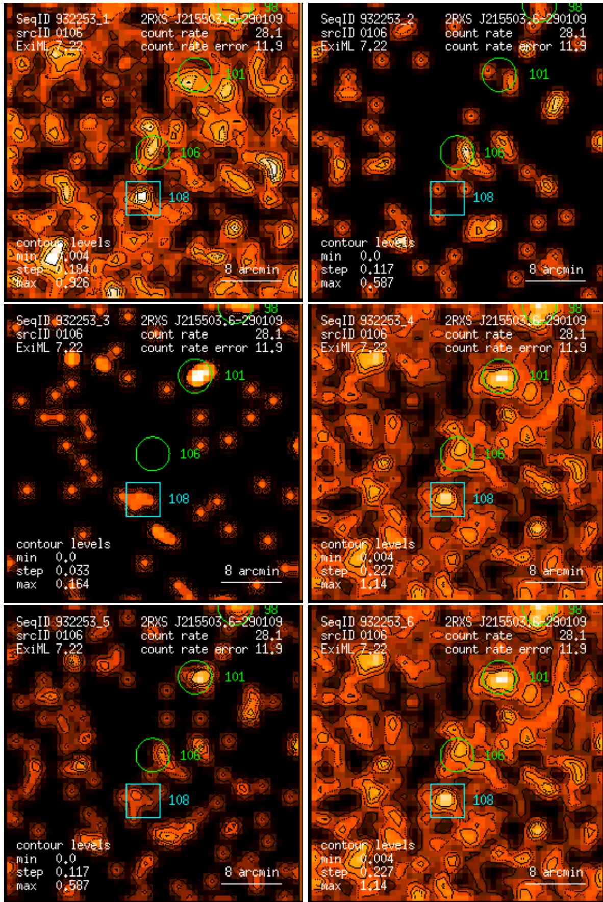
Figure 106: RASS 932253: detection 0106: band rate images, Gaussian filter: (1) PSPC channels 11 – 41, (2) 52 – 90, (3) 91 – 201, (4) 11 – 235, (5) 52 – 201, (6) 11 – 201. Broad band rates in counts/ks. Band rate contour levels in counts/ks/arcmin 2 .
