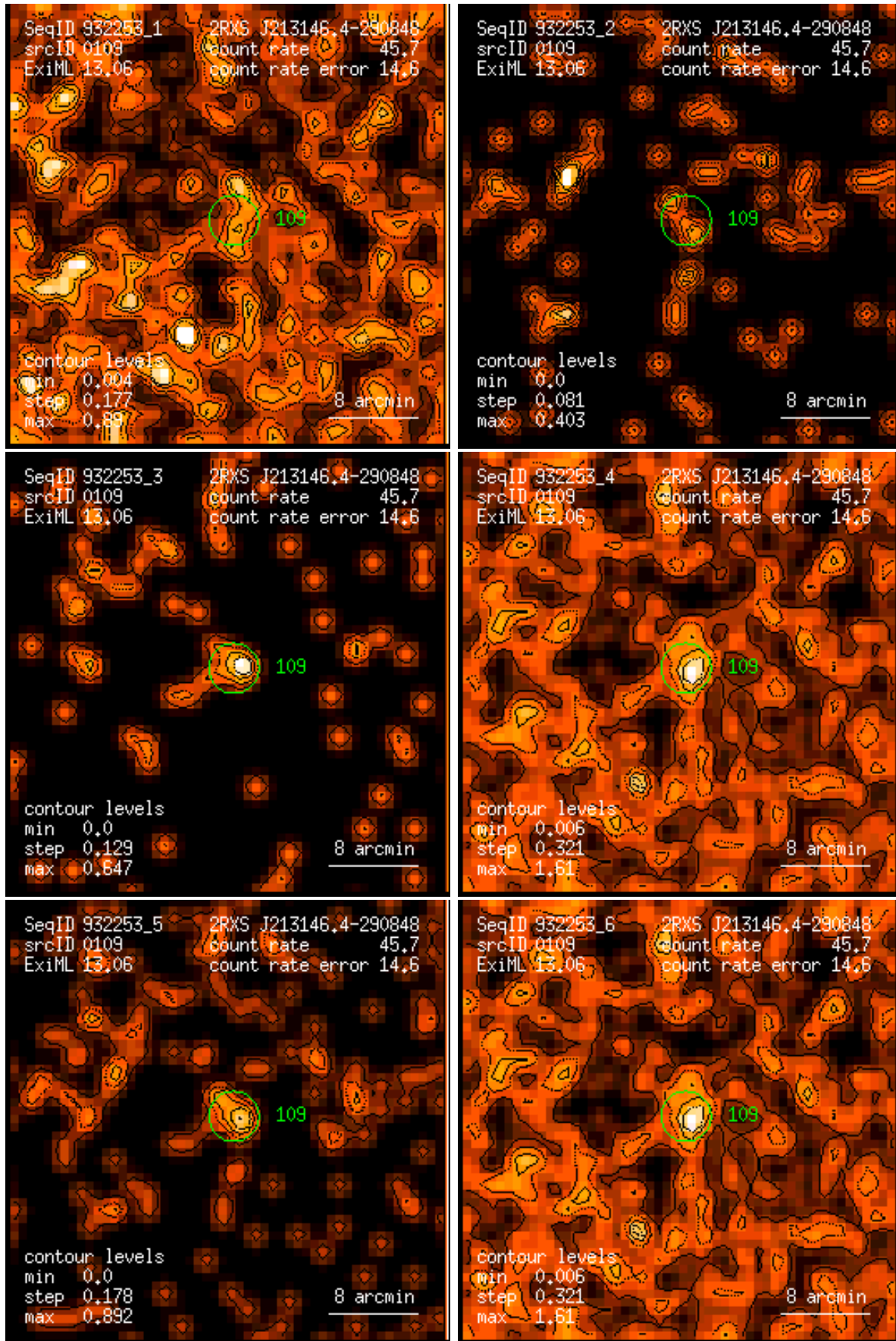
Figure 109: RASS 932253: detection 0109: band rate images, Gaussian filter: (1) PSPC channels 11 – 41, (2) 52 – 90, (3) 91 – 201, (4) 11 – 235, (5) 52 – 201, (6) 11 – 201. Broad band rates in counts/ks. Band rate contour levels in counts/ks/arcmin 2 .
