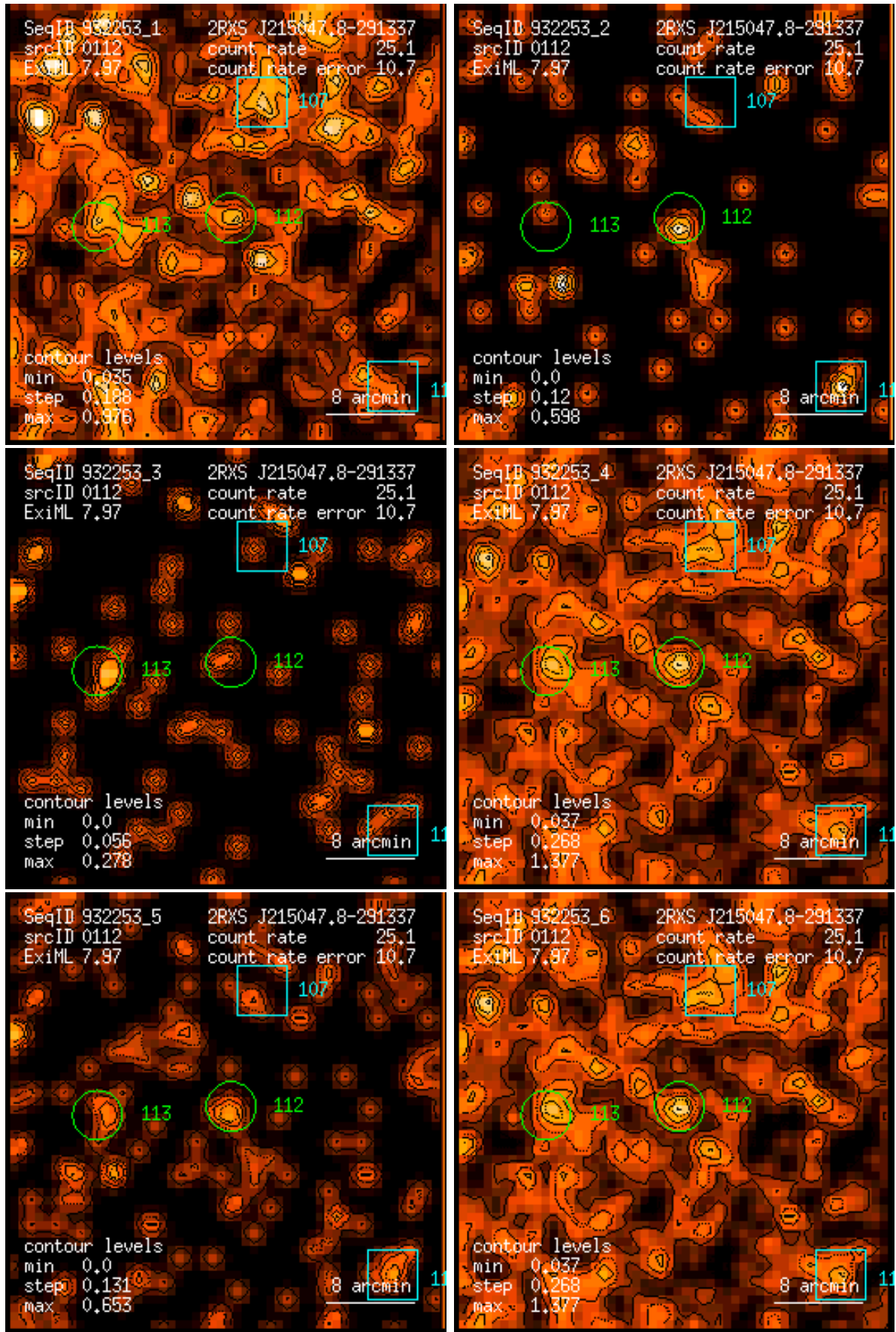
Figure 112: RASS 932253: detection 0112: band rate images, Gaussian filter: (1) PSPC channels 11 – 41, (2) 52 – 90, (3) 91 – 201, (4) 11 – 235, (5) 52 – 201, (6) 11 – 201. Broad band rates in counts/ks. Band rate contour levels in counts/ks/arcmin 2 .
