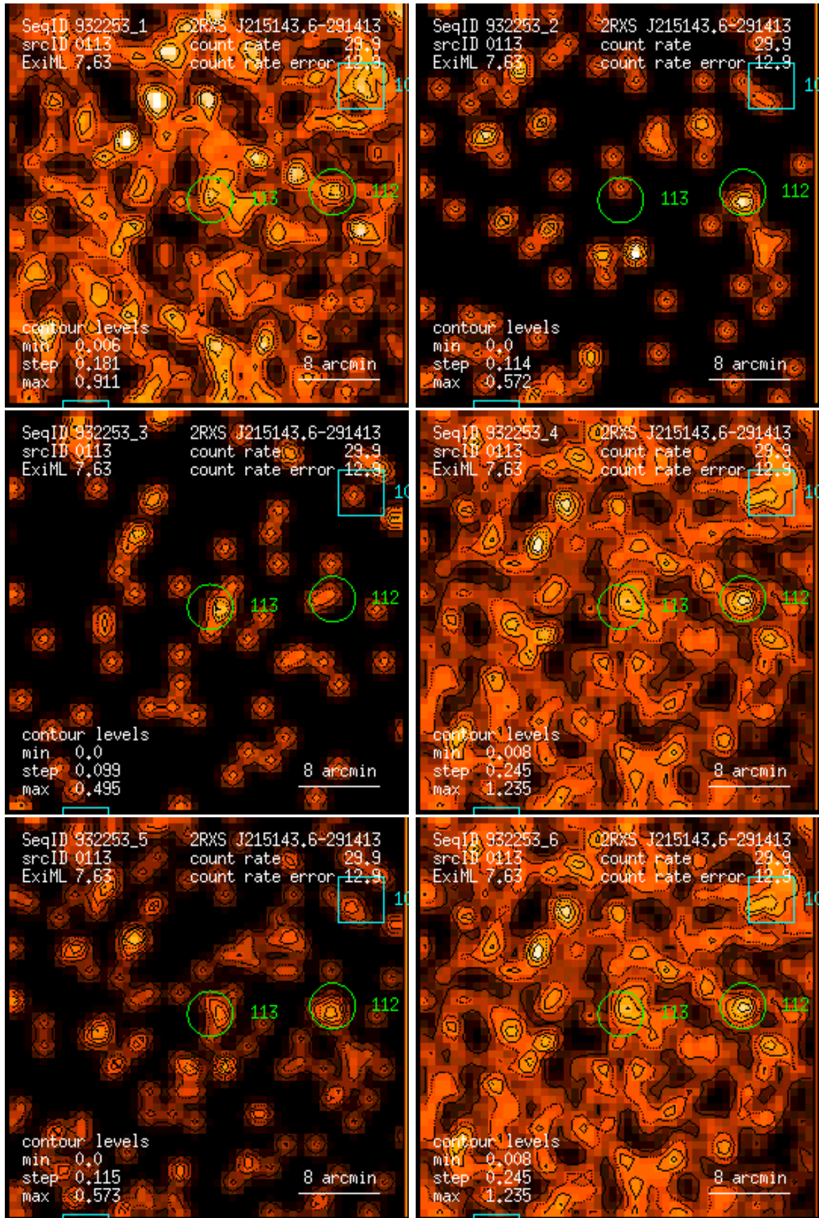
Figure 113: RASS 932253: detection 0113: band rate images, Gaussian filter: (1) PSPC channels 11 – 41, (2) 52 – 90, (3) 91 – 201, (4) 11 – 235, (5) 52 – 201, (6) 11 – 201. Broad band rates in counts/ks. Band rate contour levels in counts/ks/arcmin 2 .
