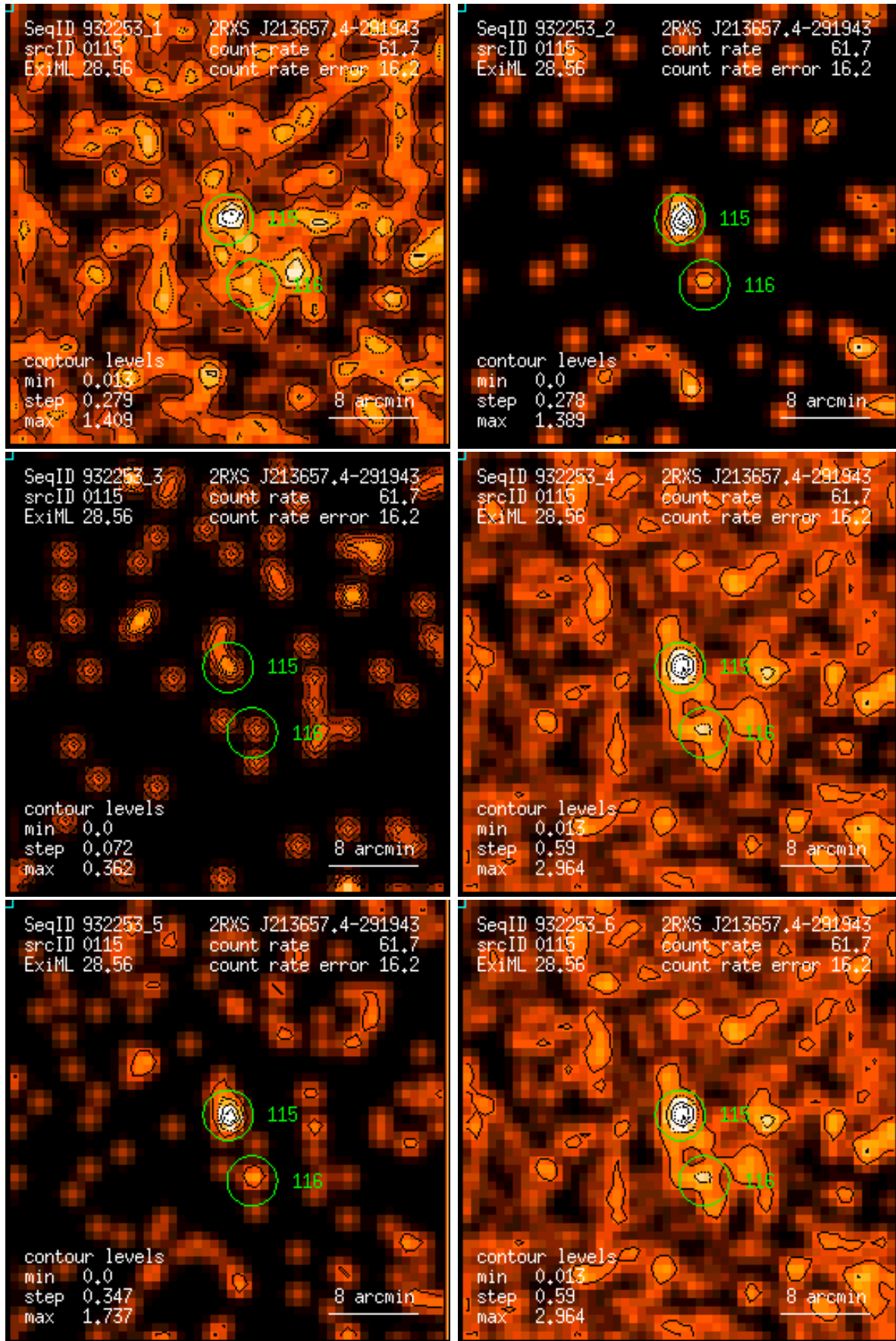
Figure 115: RASS 932253: detection 0115: band rate images, Gaussian filter: (1) PSPC channels 11 – 41, (2) 52 – 90, (3) 91 – 201, (4) 11 – 235, (5) 52 – 201, (6) 11 – 201. Broad band rates in counts/ks. Band rate contour levels in counts/ks/arcmin 2 .
