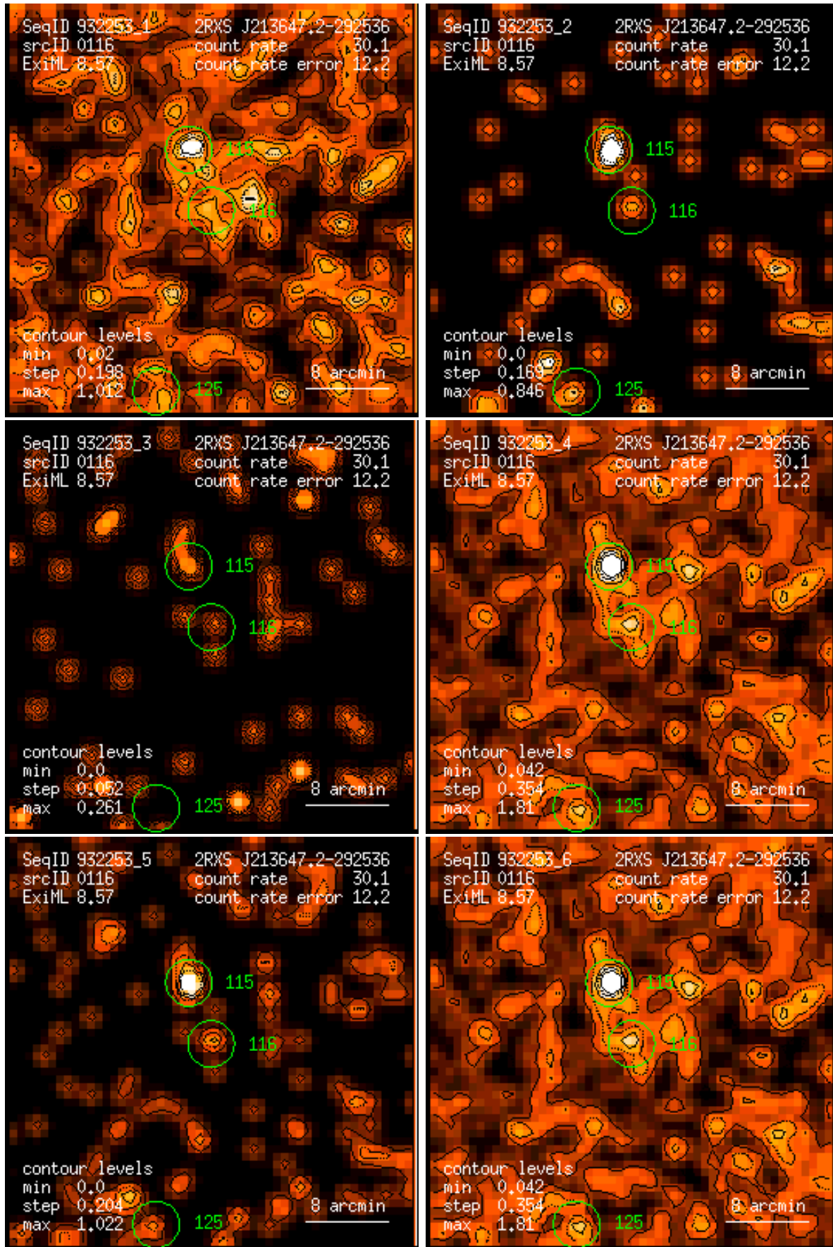
Figure 116: RASS 932253: detection 0116: band rate images, Gaussian filter: (1) PSPC channels 11 – 41, (2) 52 – 90, (3) 91 – 201, (4) 11 – 235, (5) 52 – 201, (6) 11 – 201. Broad band rates in counts/ks. Band rate contour levels in counts/ks/arcmin 2 .
