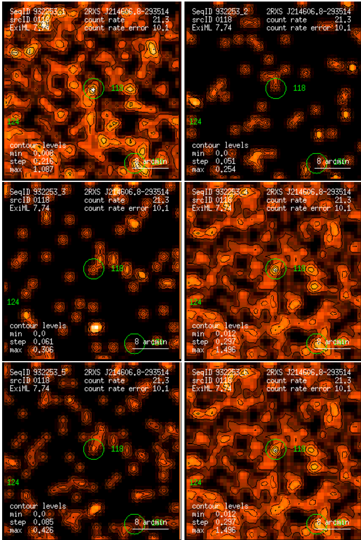
Figure 118: RASS 932253: detection 0118: band rate images, Gaussian filter: (1) PSPC channels 11 – 41, (2) 52 – 90, (3) 91 – 201, (4) 11 – 235, (5) 52 – 201, (6) 11 – 201. Broad band rates in counts/ks. Band rate contour levels in counts/ks/arcmin 2 .
