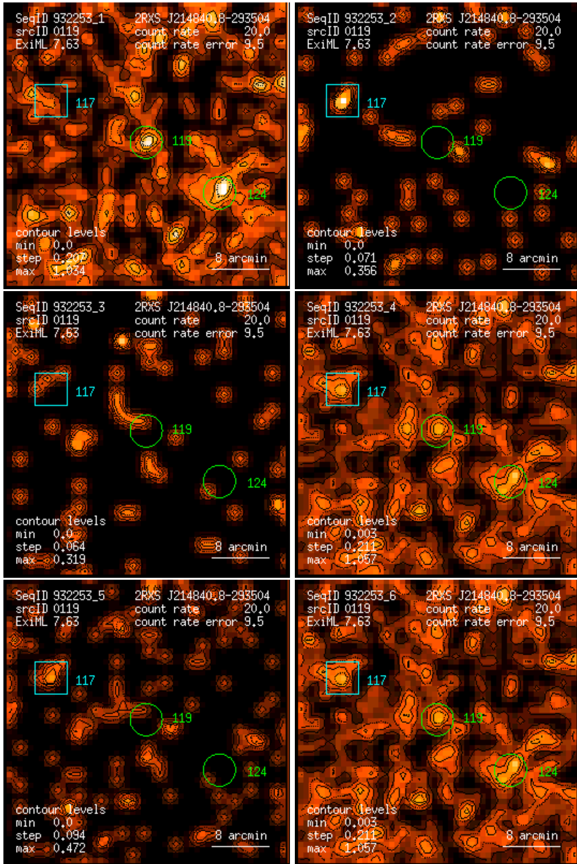
Figure 119: RASS 932253: detection 0119: band rate images, Gaussian filter: (1) PSPC channels 11 – 41, (2) 52 – 90, (3) 91 – 201, (4) 11 – 235, (5) 52 – 201, (6) 11 – 201. Broad band rates in counts/ks. Band rate contour levels in counts/ks/arcmin 2 .
