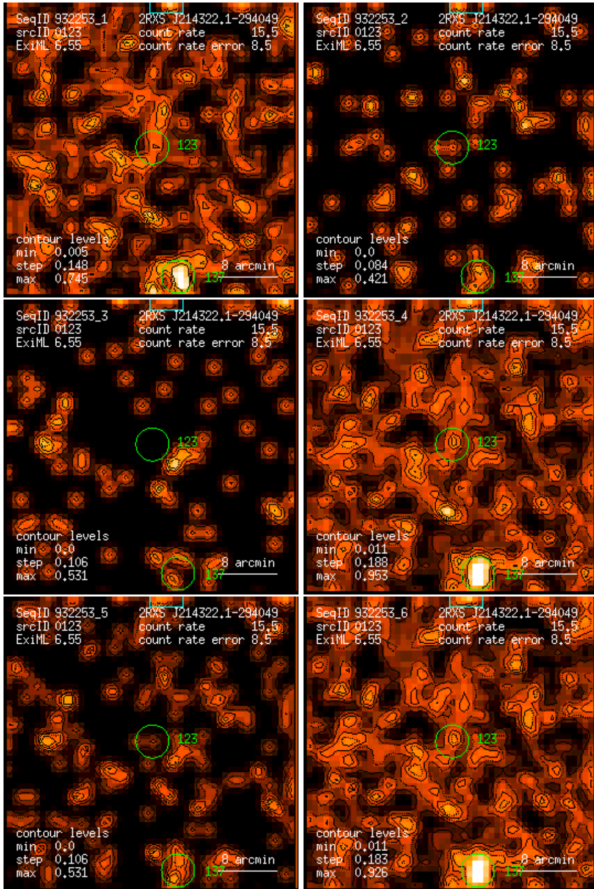
Figure 123: RASS 932253: detection 0123: band rate images, Gaussian filter: (1) PSPC channels 11 – 41, (2) 52 – 90, (3) 91 – 201, (4) 11 – 235, (5) 52 – 201, (6) 11 – 201. Broad band rates in counts/ks. Band rate contour levels in counts/ks/arcmin 2 .
