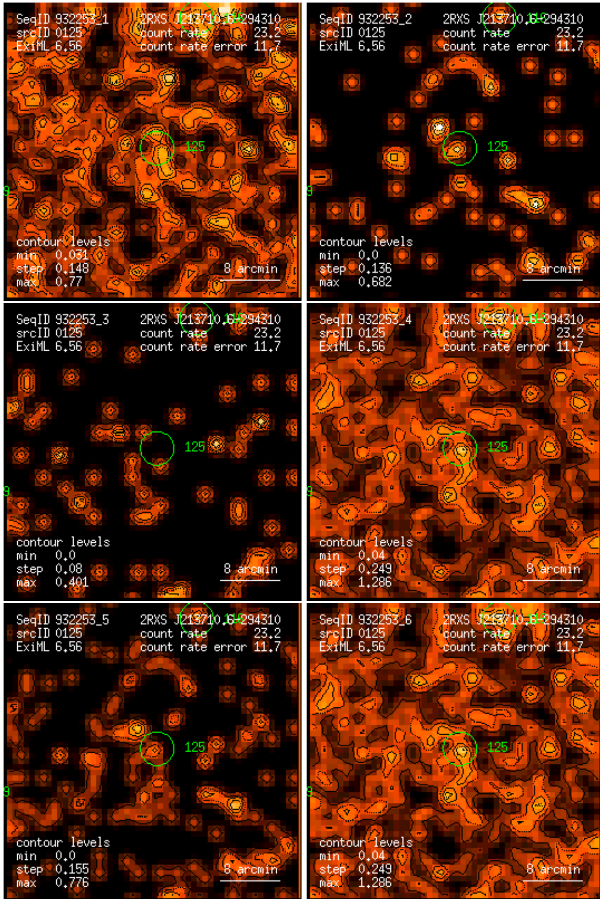
Figure 125: RASS 932253: detection 0125: band rate images, Gaussian filter: (1) PSPC channels 11 – 41, (2) 52 – 90, (3) 91 – 201, (4) 11 – 235, (5) 52 – 201, (6) 11 – 201. Broad band rates in counts/ks. Band rate contour levels in counts/ks/arcmin 2 .
