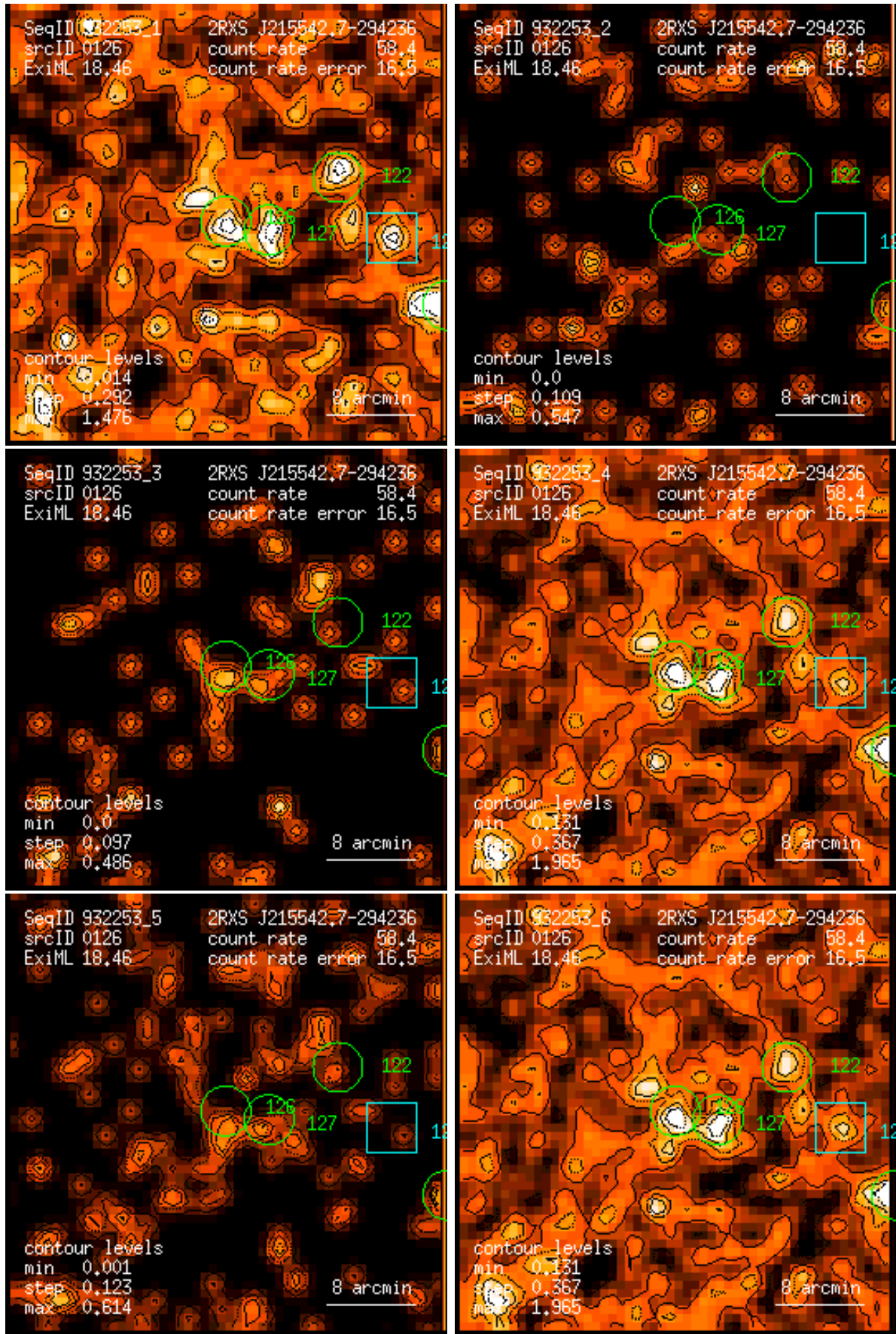
Figure 126: RASS 932253: detection 0126: band rate images, Gaussian filter: (1) PSPC channels 11 – 41, (2) 52 – 90, (3) 91 – 201, (4) 11 – 235, (5) 52 – 201, (6) 11 – 201. Broad band rates in counts/ks. Band rate contour levels in counts/ks/arcmin 2 .
