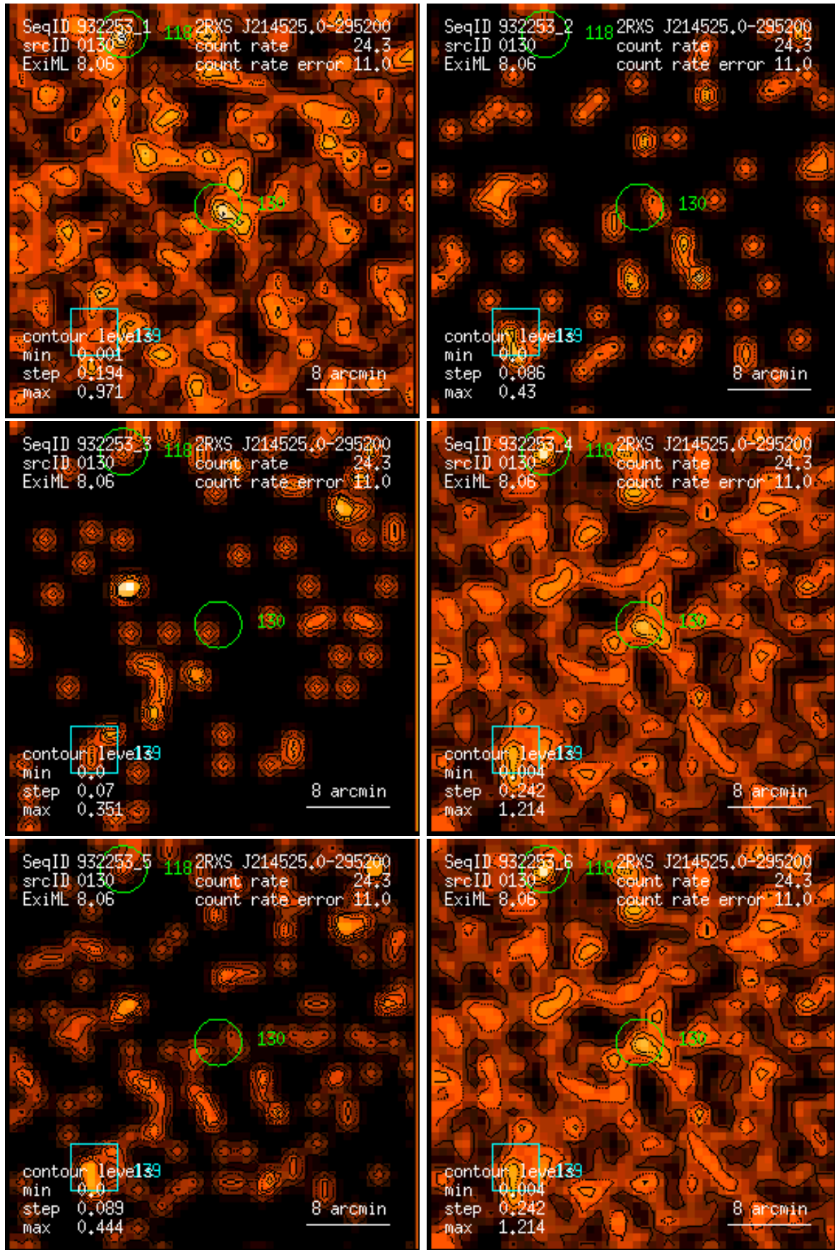
Figure 130: RASS 932253: detection 0130: band rate images, Gaussian filter: (1) PSPC channels 11 – 41, (2) 52 – 90, (3) 91 – 201, (4) 11 – 235, (5) 52 – 201, (6) 11 – 201. Broad band rates in counts/ks. Band rate contour levels in counts/ks/arcmin 2 .
