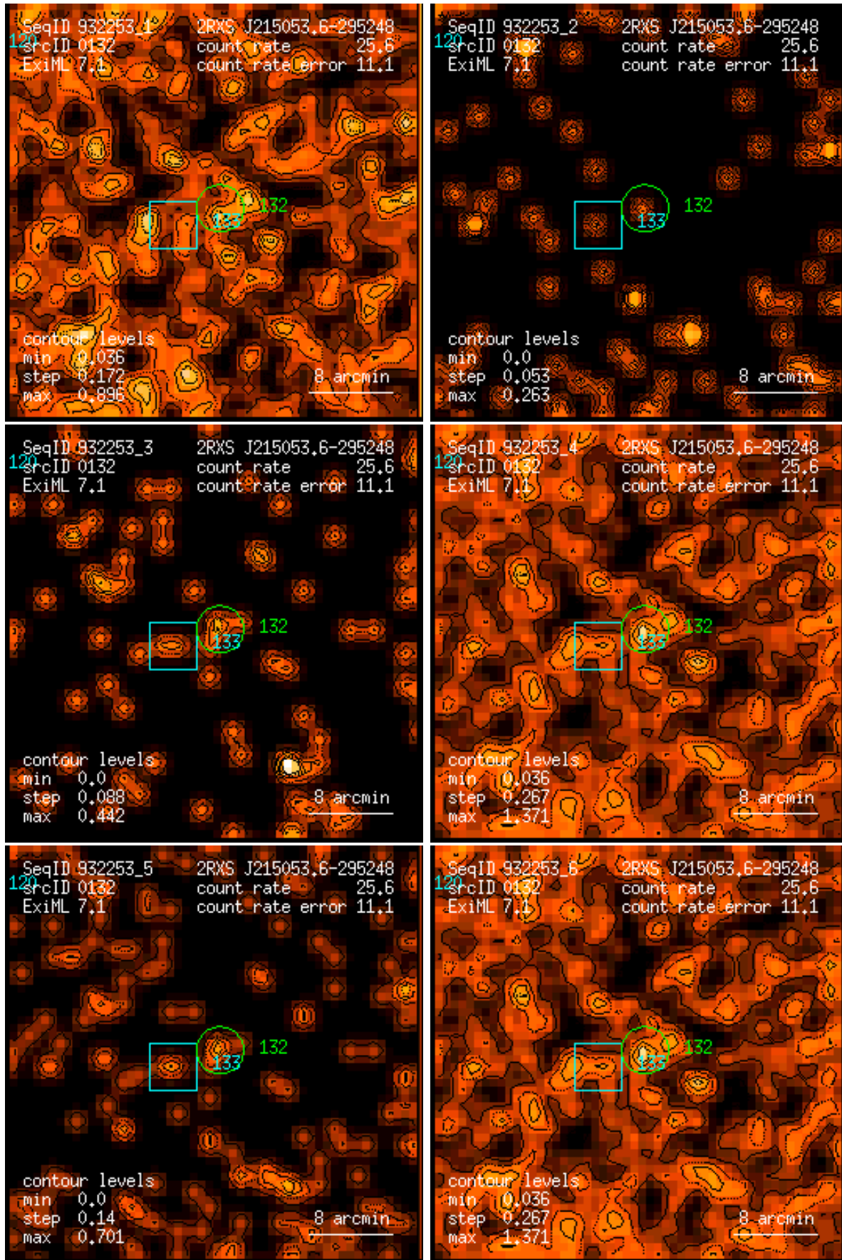
Figure 132: RASS 932253: detection 0132: band rate images, Gaussian filter: (1) PSPC channels 11 – 41, (2) 52 – 90, (3) 91 – 201, (4) 11 – 235, (5) 52 – 201, (6) 11 – 201. Broad band rates in counts/ks. Band rate contour levels in counts/ks/arcmin 2 .
