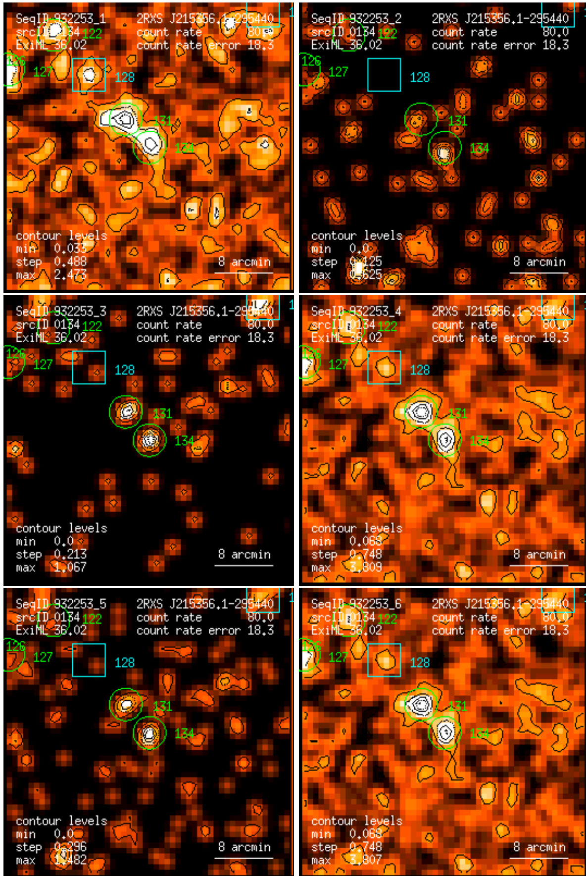
Figure 134: RASS 932253: detection 0134: band rate images, Gaussian filter: (1) PSPC channels 11 – 41, (2) 52 – 90, (3) 91 – 201, (4) 11 – 235, (5) 52 – 201, (6) 11 – 201. Broad band rates in counts/ks. Band rate contour levels in counts/ks/arcmin 2 .
