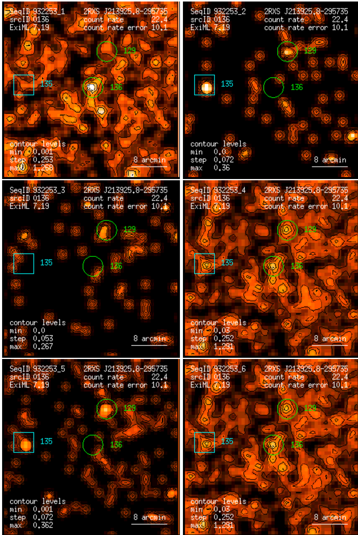
Figure 136: RASS 932253: detection 0136: band rate images, Gaussian filter: (1) PSPC channels 11 – 41, (2) 52 – 90, (3) 91 – 201, (4) 11 – 235, (5) 52 – 201, (6) 11 – 201. Broad band rates in counts/ks. Band rate contour levels in counts/ks/arcmin 2 .
