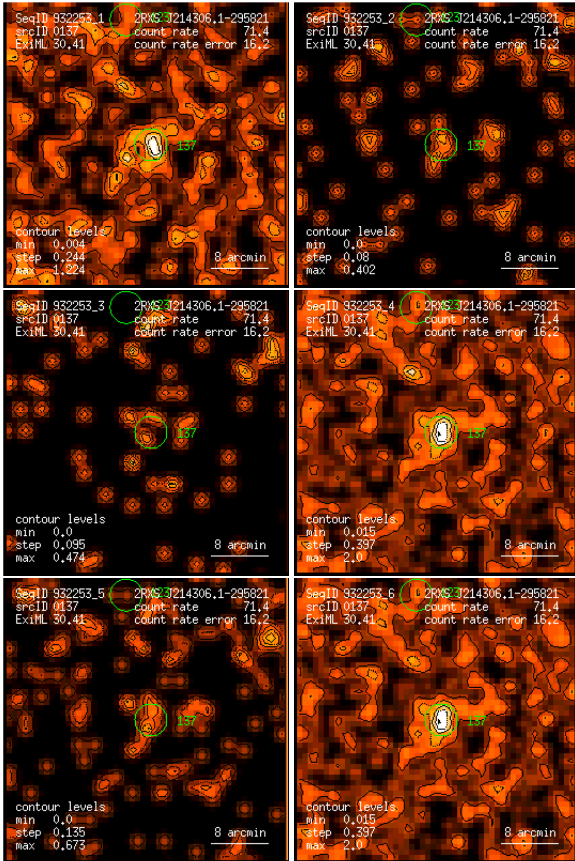
Figure 137: RASS 932253: detection 0137: band rate images, Gaussian filter: (1) PSPC channels 11 – 41, (2) 52 – 90, (3) 91 – 201, (4) 11 – 235, (5) 52 – 201, (6) 11 – 201. Broad band rates in counts/ks. Band rate contour levels in counts/ks/arcmin 2 .
