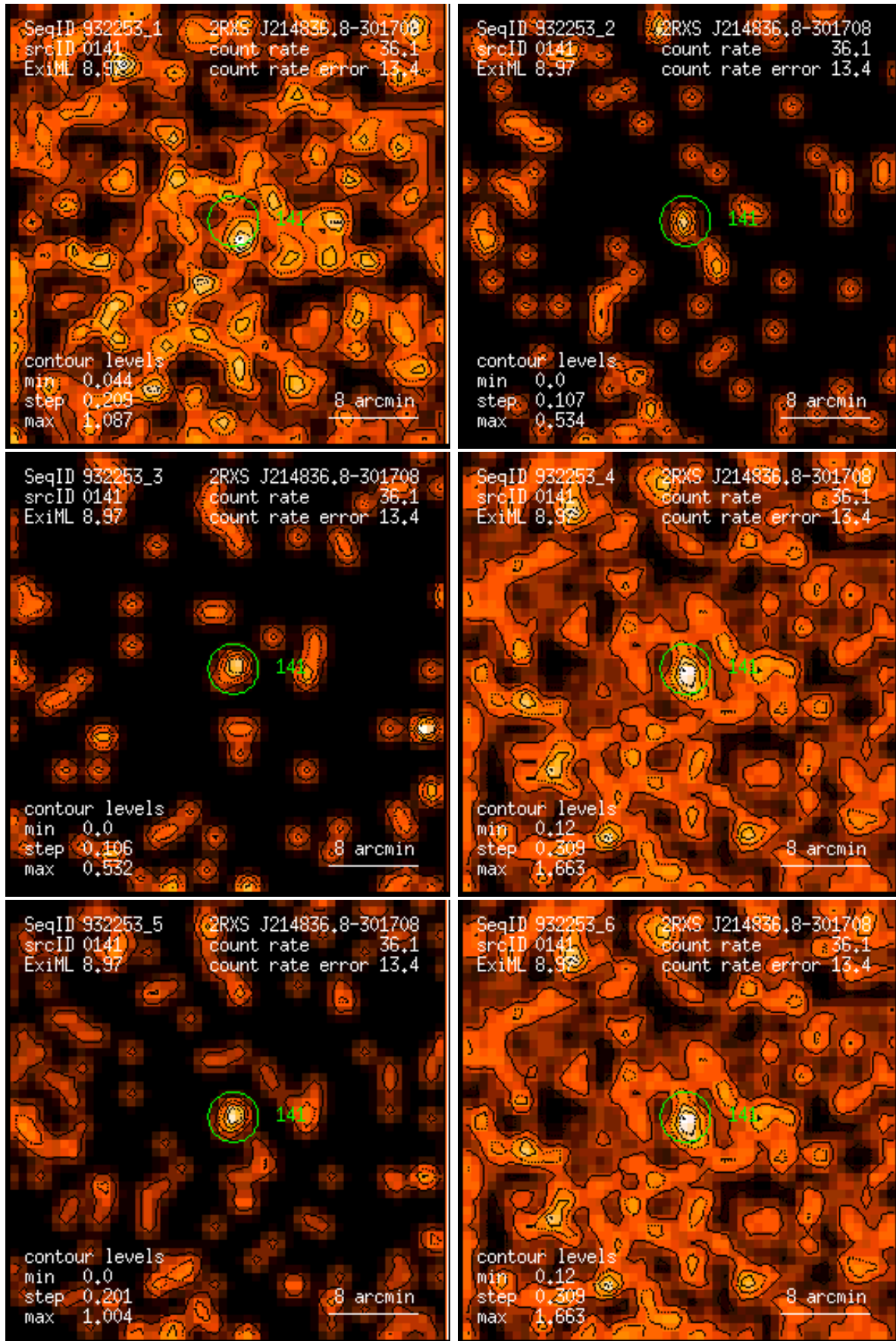
Figure 141: RASS 932253: detection 0141: band rate images, Gaussian filter: (1) PSPC channels 11 – 41, (2) 52 – 90, (3) 91 – 201, (4) 11 – 235, (5) 52 – 201, (6) 11 – 201. Broad band rates in counts/ks. Band rate contour levels in counts/ks/arcmin 2 .
