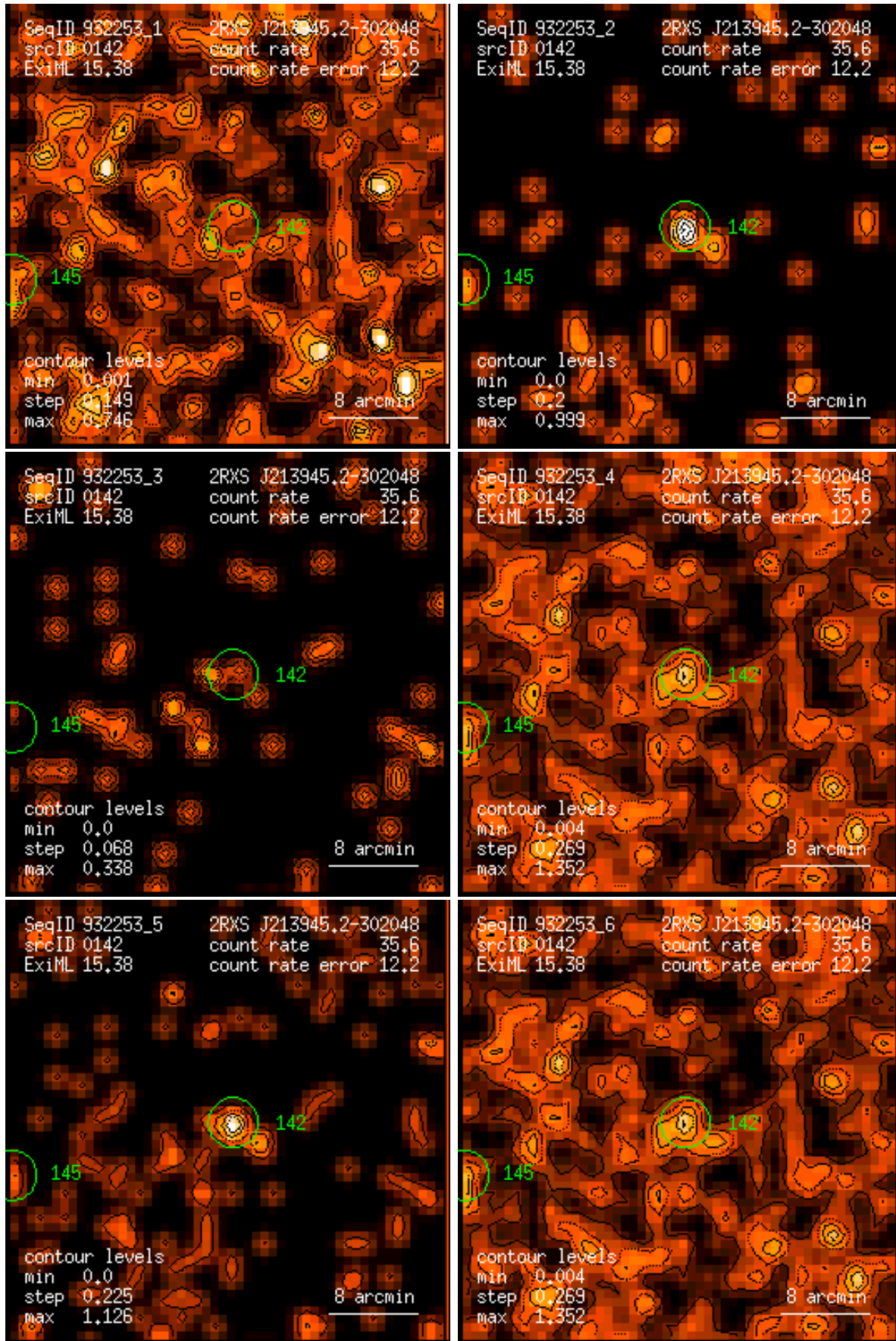
Figure 142: RASS 932253: detection 0142: band rate images, Gaussian filter: (1) PSPC channels 11 – 41, (2) 52 – 90, (3) 91 – 201, (4) 11 – 235, (5) 52 – 201, (6) 11 – 201. Broad band rates in counts/ks. Band rate contour levels in counts/ks/arcmin 2 .
