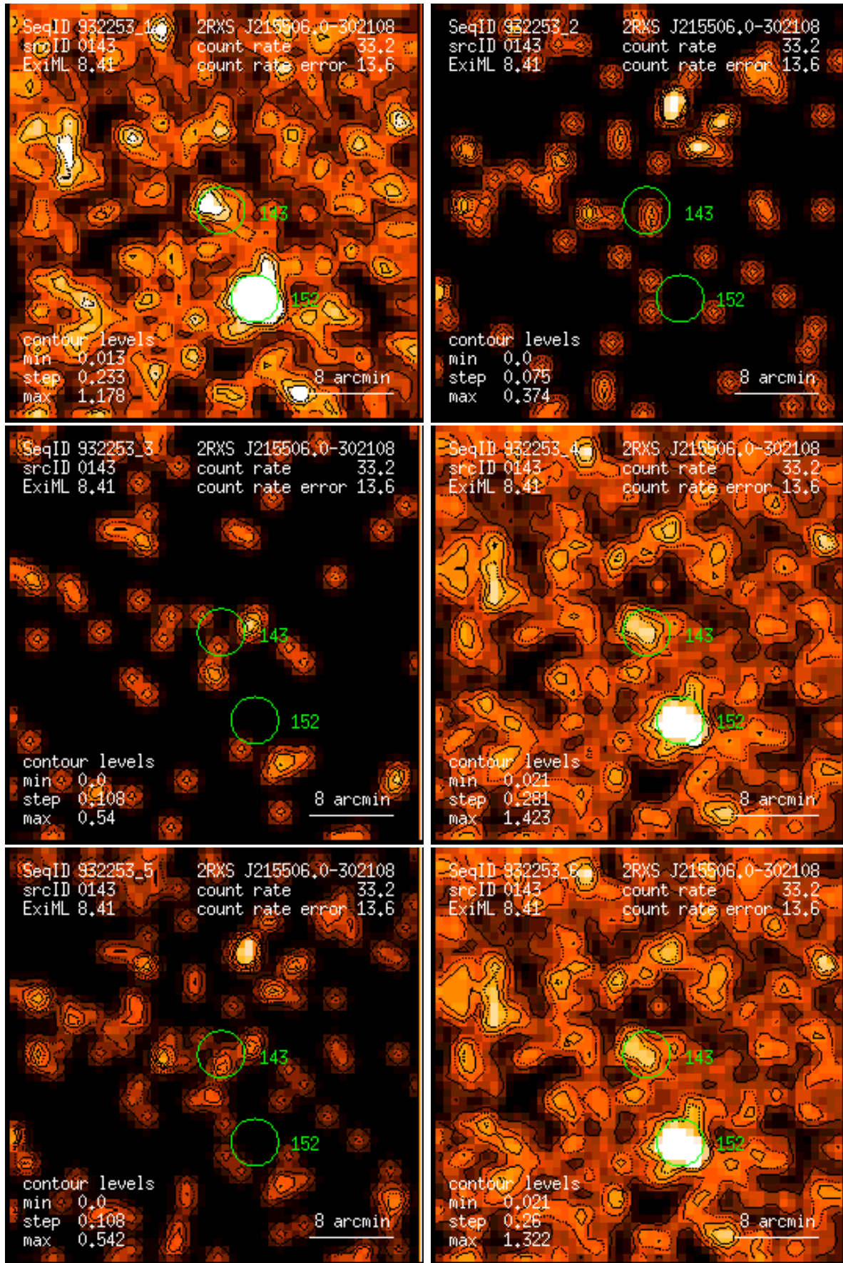
Figure 143: RASS 932253: detection 0143: band rate images, Gaussian filter: (1) PSPC channels 11 – 41, (2) 52 – 90, (3) 91 – 201, (4) 11 – 235, (5) 52 – 201, (6) 11 – 201. Broad band rates in counts/ks. Band rate contour levels in counts/ks/arcmin 2 .
