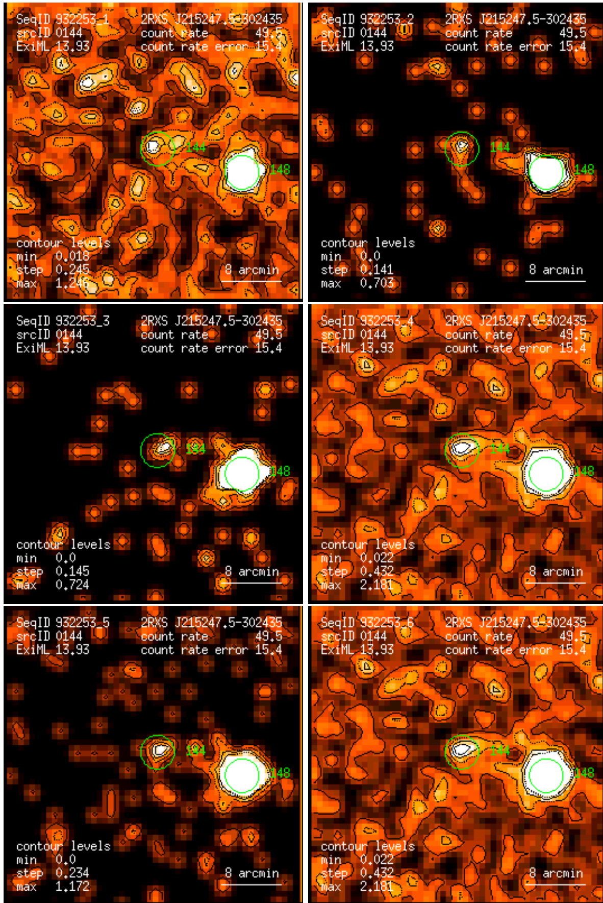
Figure 144: RASS 932253: detection 0144: band rate images, Gaussian filter: (1) PSPC channels 11 – 41, (2) 52 – 90, (3) 91 – 201, (4) 11 – 235, (5) 52 – 201, (6) 11 – 201. Broad band rates in counts/ks. Band rate contour levels in counts/ks/arcmin 2 .
