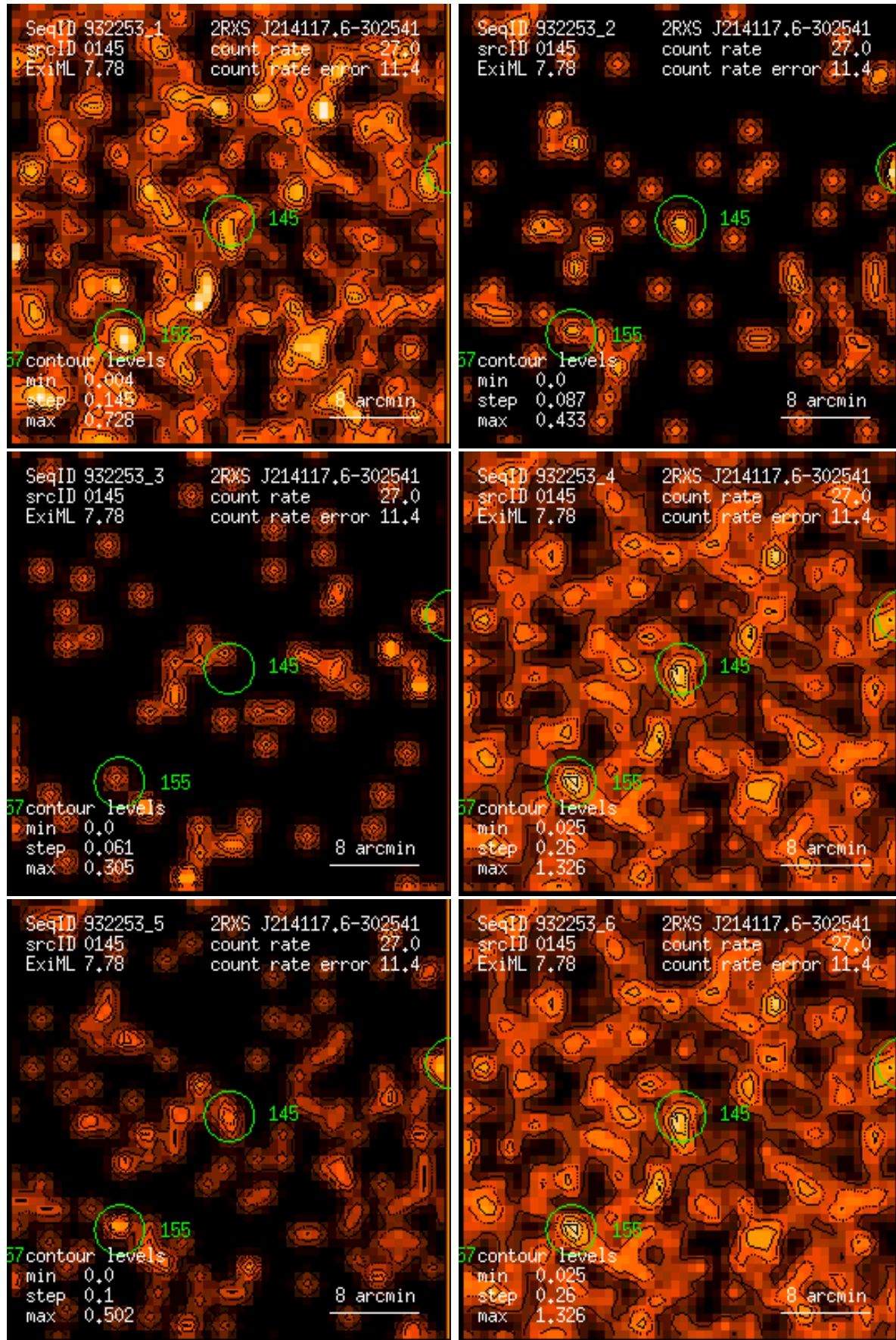
Figure 145: RASS 932253: detection 0145: band rate images, Gaussian filter: (1) PSPC channels 11 – 41, (2) 52 – 90, (3) 91 – 201, (4) 11 – 235, (5) 52 – 201, (6) 11 – 201. Broad band rates in counts/ks. Band rate contour levels in counts/ks/arcmin 2 .
