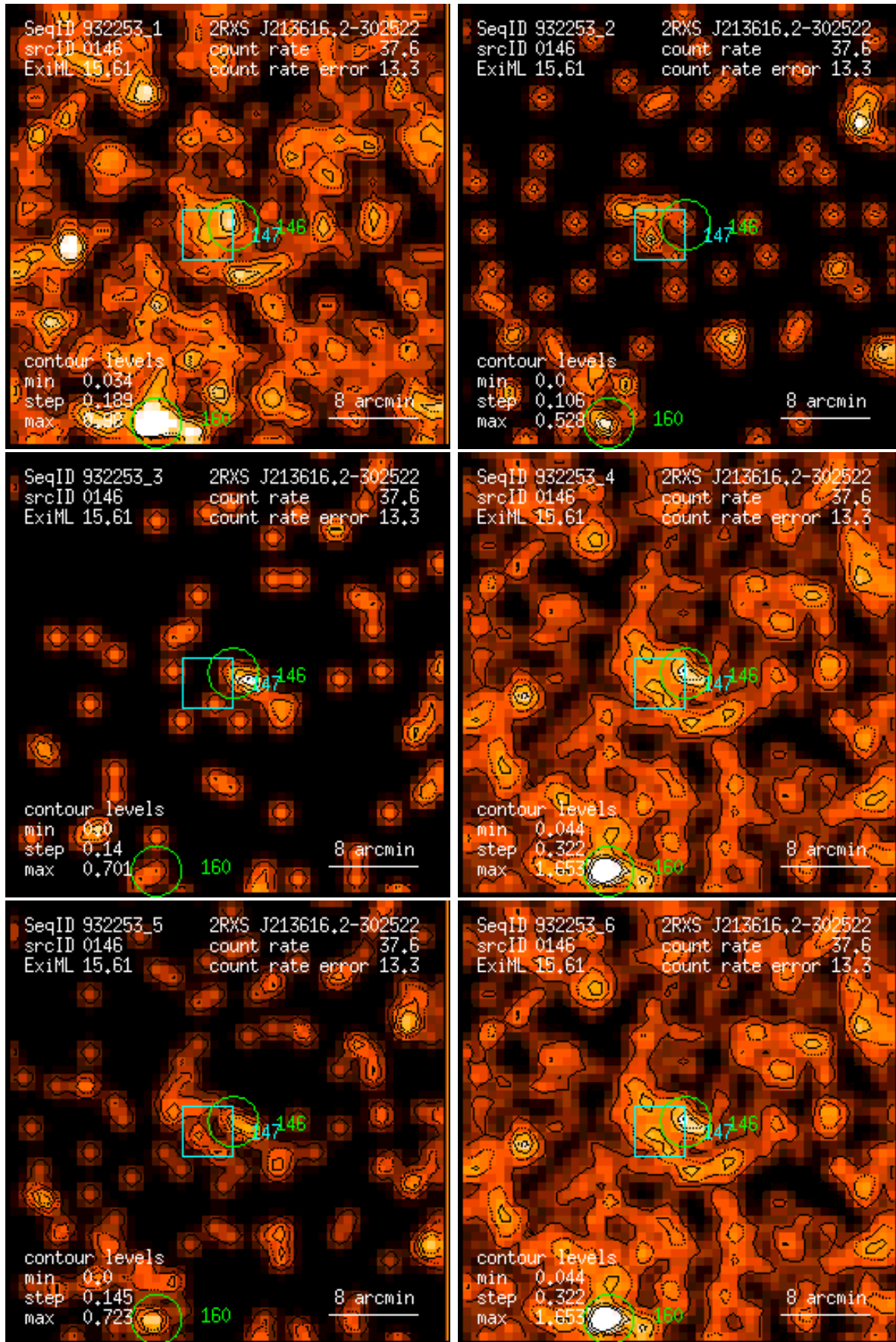
Figure 146: RASS 932253: detection 0146: band rate images, Gaussian filter: (1) PSPC channels 11 – 41, (2) 52 – 90, (3) 91 – 201, (4) 11 – 235, (5) 52 – 201, (6) 11 – 201. Broad band rates in counts/ks. Band rate contour levels in counts/ks/arcmin 2 .
