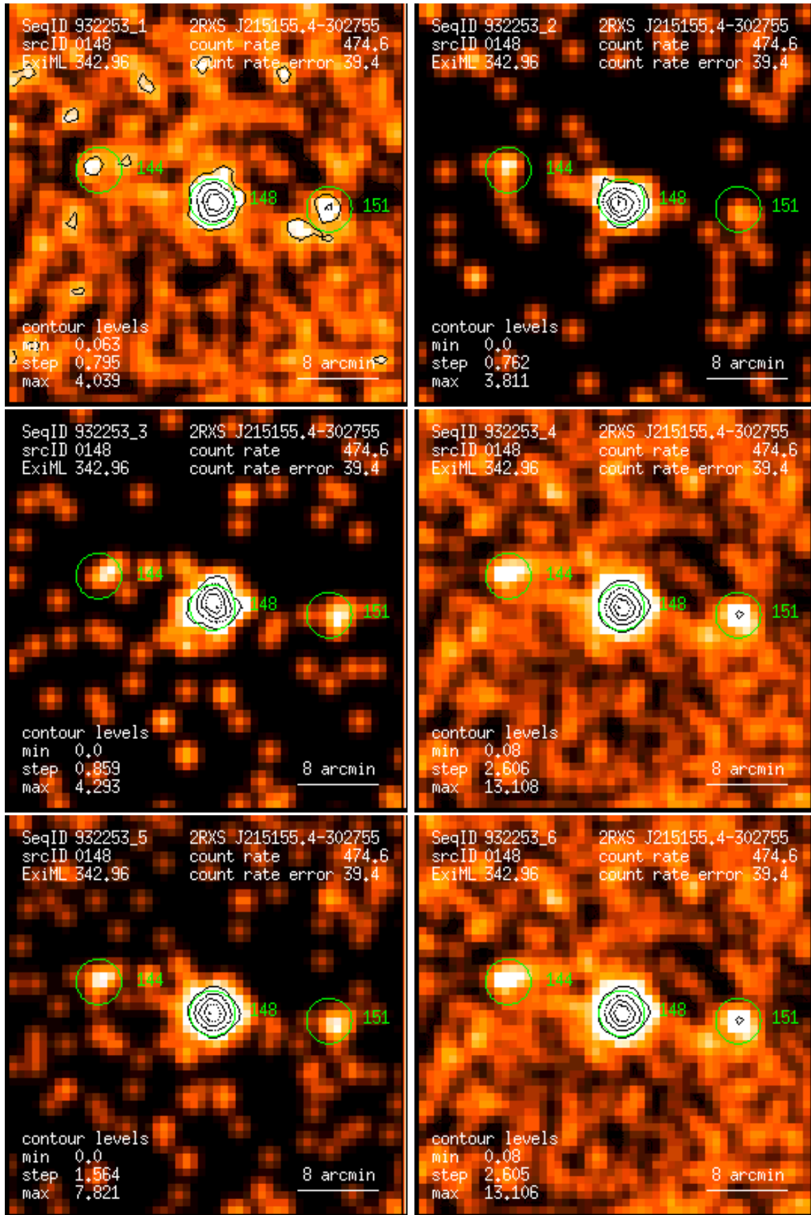
Figure 148: RASS 932253: detection 0148: band rate images, Gaussian filter: (1) PSPC channels 11 – 41, (2) 52 – 90, (3) 91 – 201, (4) 11 – 235, (5) 52 – 201, (6) 11 – 201. Broad band rates in counts/ks. Band rate contour levels in counts/ks/arcmin 2 .
