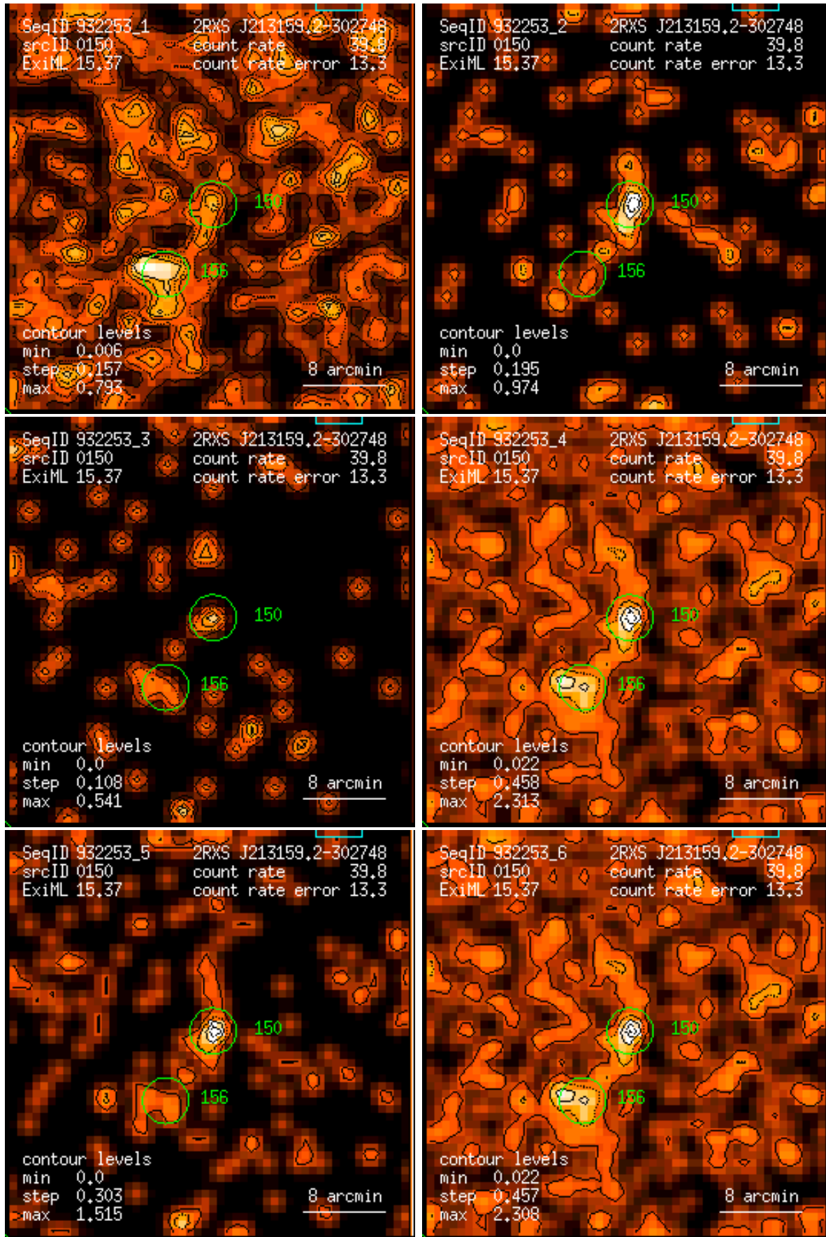
Figure 150: RASS 932253: detection 0150: band rate images, Gaussian filter: (1) PSPC channels 11 – 41, (2) 52 – 90, (3) 91 – 201, (4) 11 – 235, (5) 52 – 201, (6) 11 – 201. Broad band rates in counts/ks. Band rate contour levels in counts/ks/arcmin 2 .
