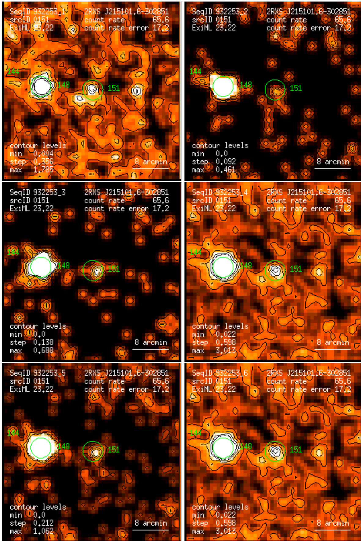
Figure 151: RASS 932253: detection 0151: band rate images, Gaussian filter: (1) PSPC channels 11 – 41, (2) 52 – 90, (3) 91 – 201, (4) 11 – 235, (5) 52 – 201, (6) 11 – 201. Broad band rates in counts/ks. Band rate contour levels in counts/ks/arcmin 2 .
