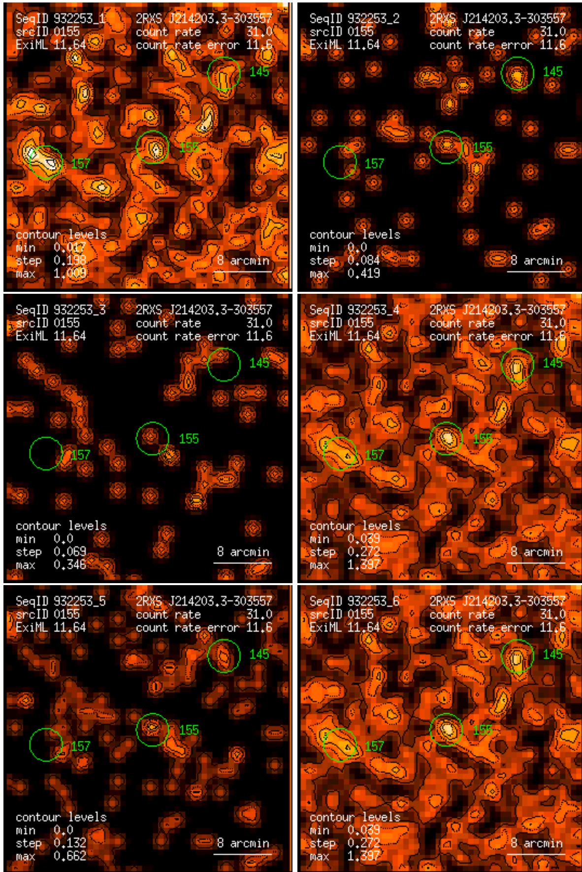
Figure 155: RASS 932253: detection 0155: band rate images, Gaussian filter: (1) PSPC channels 11 – 41, (2) 52 – 90, (3) 91 – 201, (4) 11 – 235, (5) 52 – 201, (6) 11 – 201. Broad band rates in counts/ks. Band rate contour levels in counts/ks/arcmin 2 .
