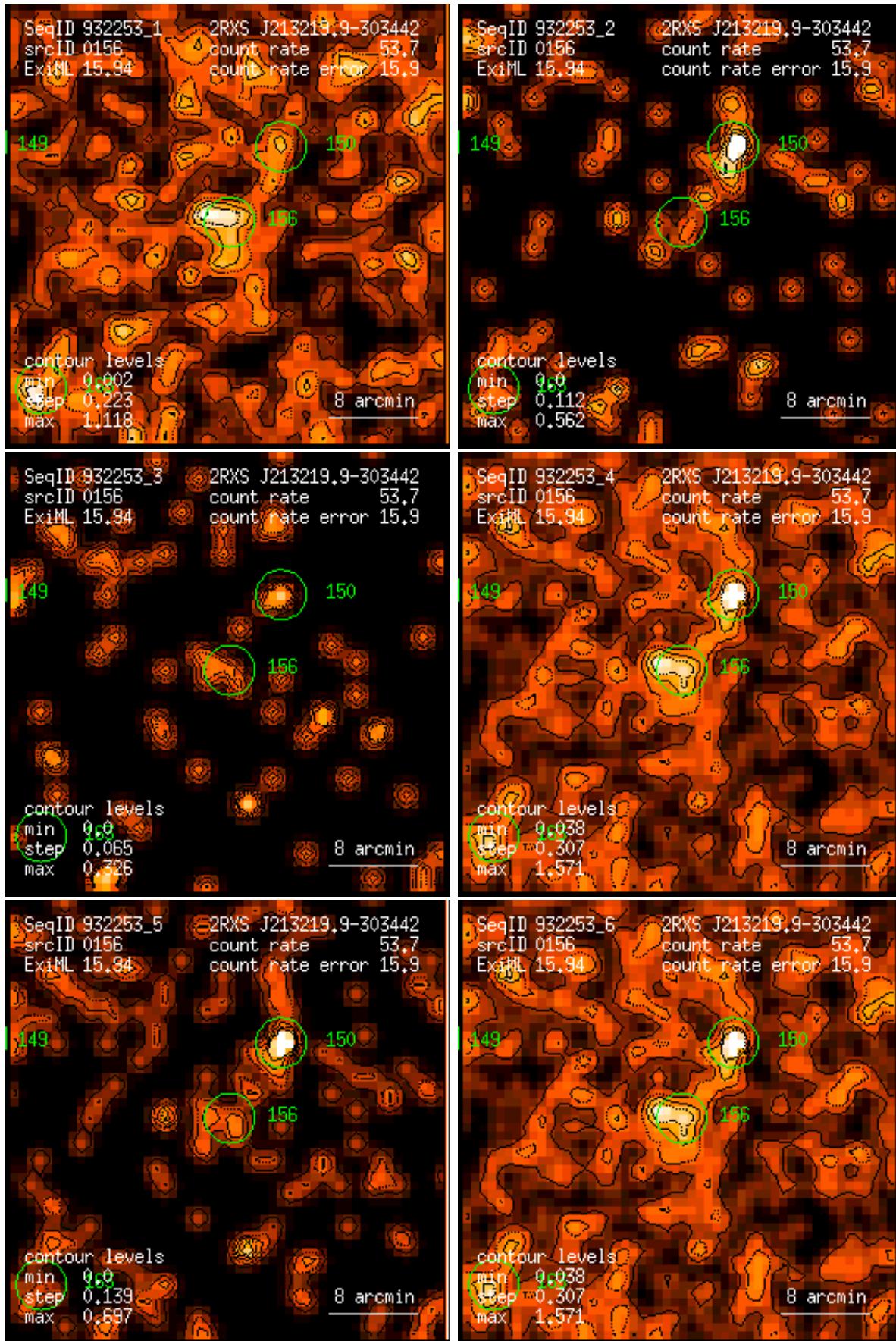
Figure 156: RASS 932253: detection 0156: band rate images, Gaussian filter: (1) PSPC channels 11 – 41, (2) 52 – 90, (3) 91 – 201, (4) 11 – 235, (5) 52 – 201, (6) 11 – 201. Broad band rates in counts/ks. Band rate contour levels in counts/ks/arcmin 2 .
