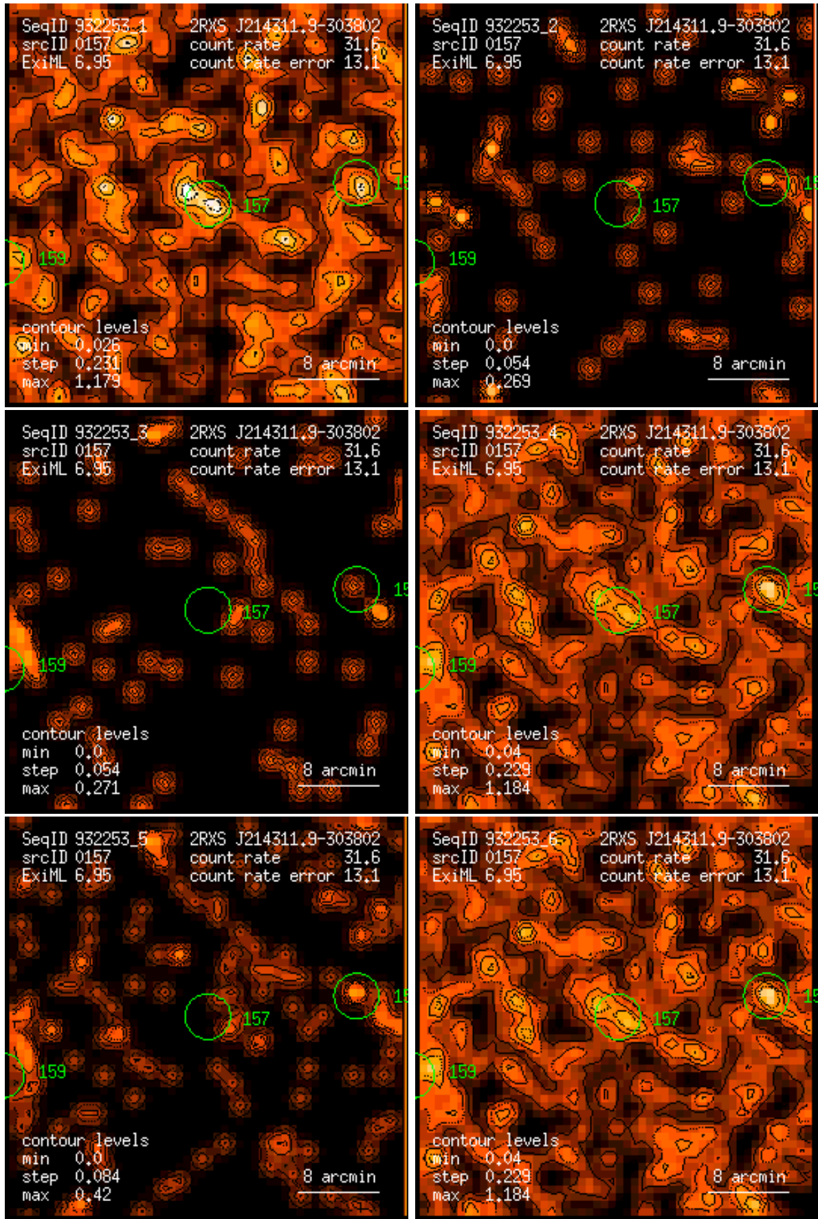
Figure 157: RASS 932253: detection 0157: band rate images, Gaussian filter: (1) PSPC channels 11 – 41, (2) 52 – 90, (3) 91 – 201, (4) 11 – 235, (5) 52 – 201, (6) 11 – 201. Broad band rates in counts/ks. Band rate contour levels in counts/ks/arcmin 2 .
