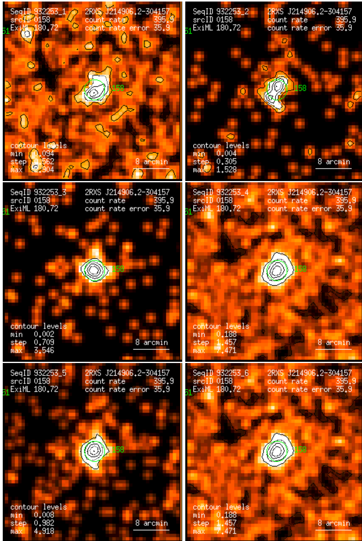
Figure 158: RASS 932253: detection 0158: band rate images, Gaussian filter: (1) PSPC channels 11 – 41, (2) 52 – 90, (3) 91 – 201, (4) 11 – 235, (5) 52 – 201, (6) 11 – 201. Broad band rates in counts/ks. Band rate contour levels in counts/ks/arcmin 2 .
