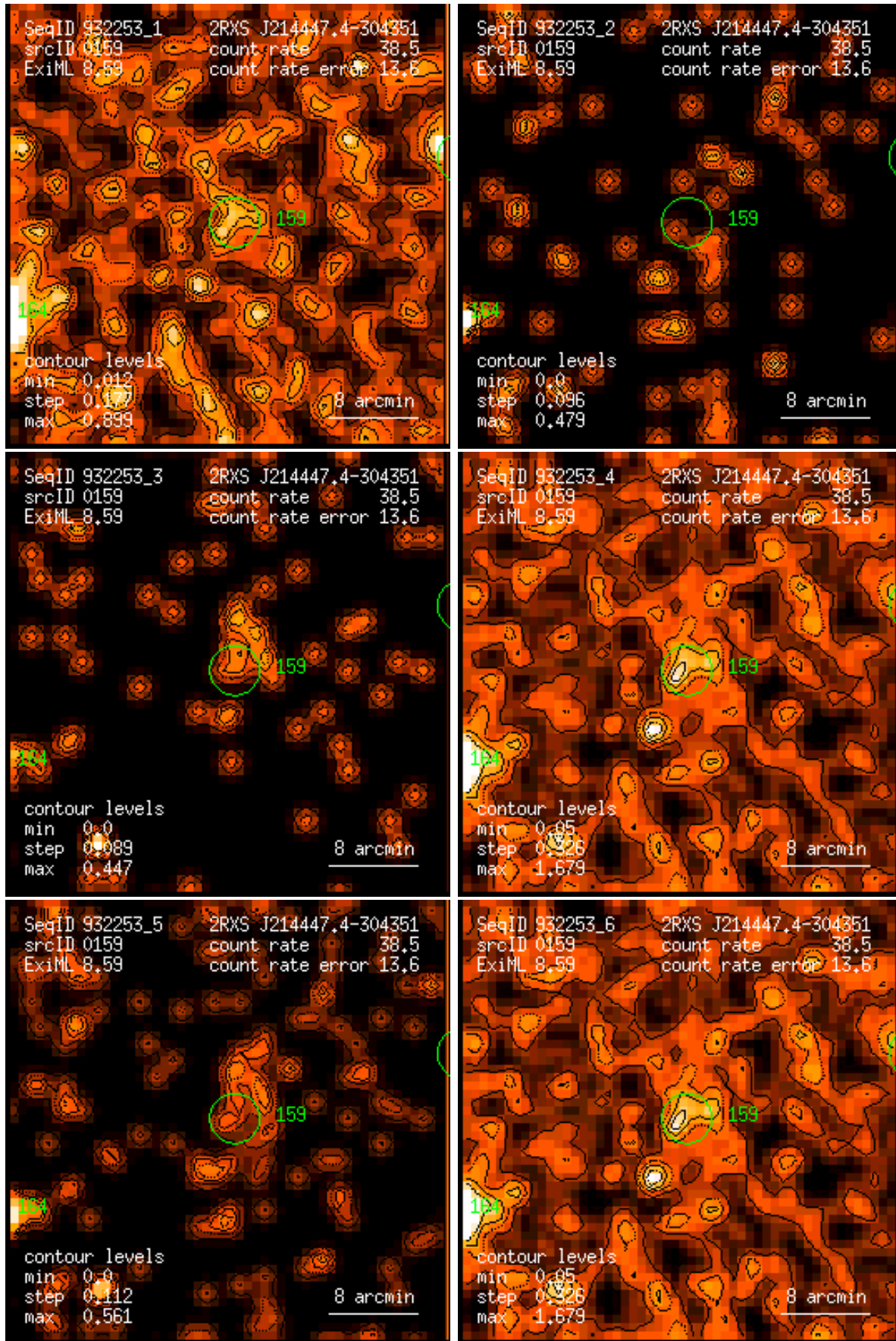
Figure 159: RASS 932253: detection 0159: band rate images, Gaussian filter: (1) PSPC channels 11 – 41, (2) 52 – 90, (3) 91 – 201, (4) 11 – 235, (5) 52 – 201, (6) 11 – 201. Broad band rates in counts/ks. Band rate contour levels in counts/ks/arcmin 2 .
