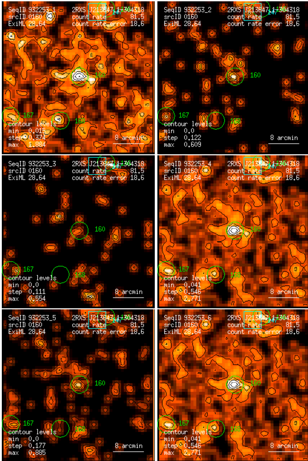
Figure 160: RASS 932253: detection 0160: band rate images, Gaussian filter: (1) PSPC channels 11 – 41, (2) 52 – 90, (3) 91 – 201, (4) 11 – 235, (5) 52 – 201, (6) 11 – 201. Broad band rates in counts/ks. Band rate contour levels in counts/ks/arcmin 2 .
